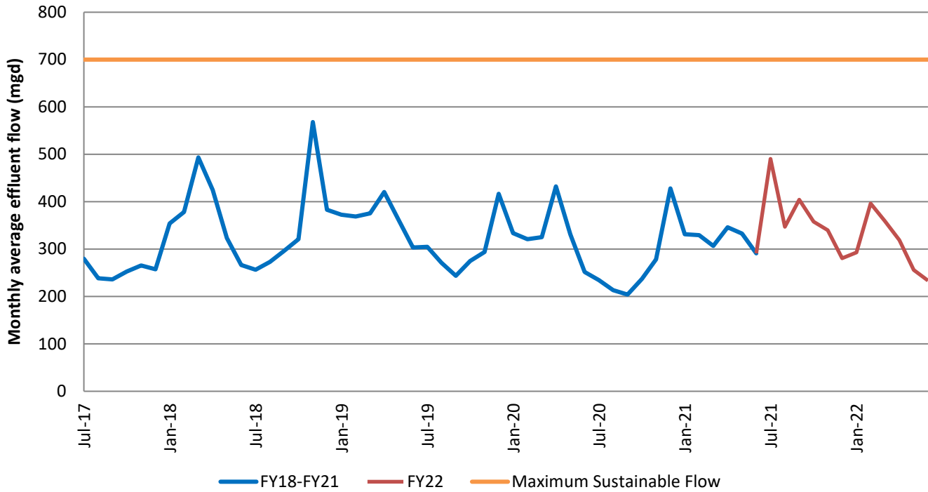
Figure 5. Average Monthly Flow
