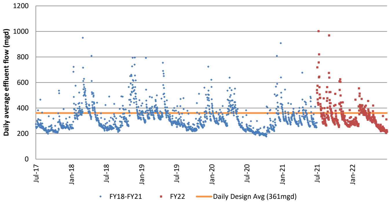
Figure 4. Average Daily Flow
