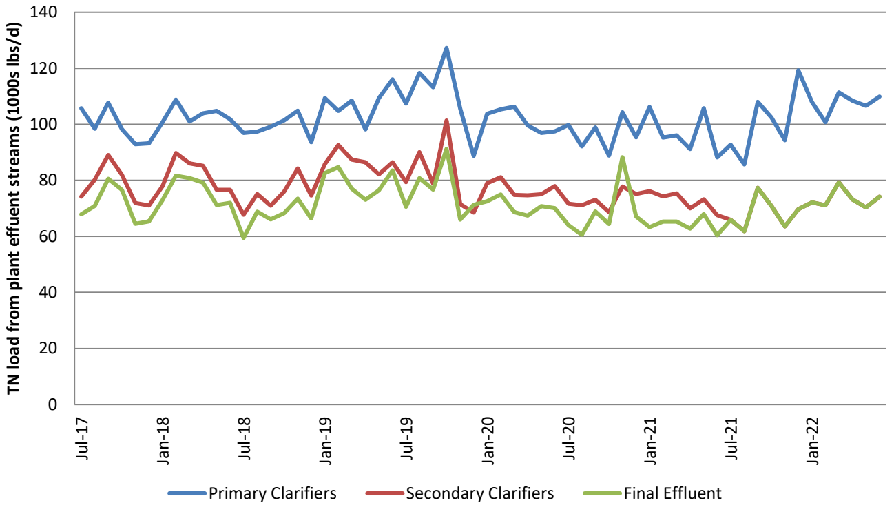
Figure 8. Total Nitrogen Load From Plant Effluent Streams
