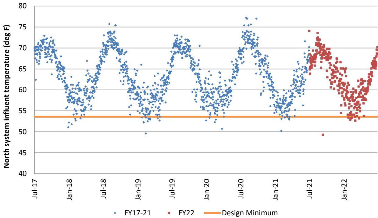
Figure 9. North System Influent Temperatures
