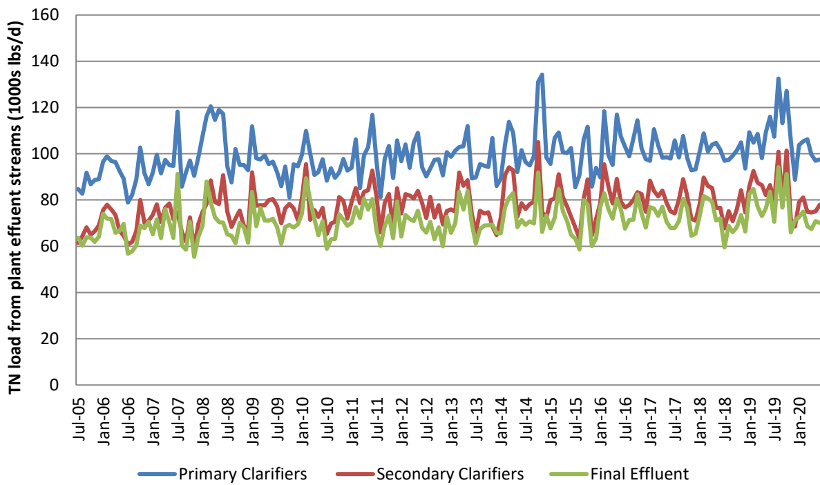
Figure 8. Total Nitrogen Load From Plant Effluent Streams
