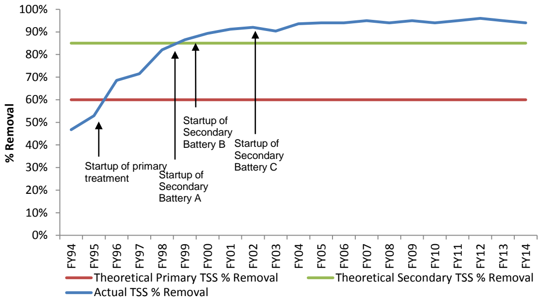
Figure 3. DITP Effluent TSS Removal Rate, FY94-FY14
