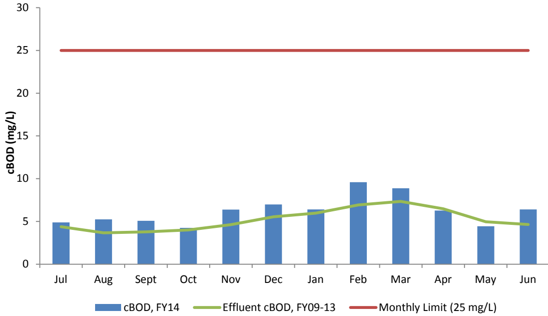
Figure 16. DITP Effluent cBOD (Monthly Average), FY14
