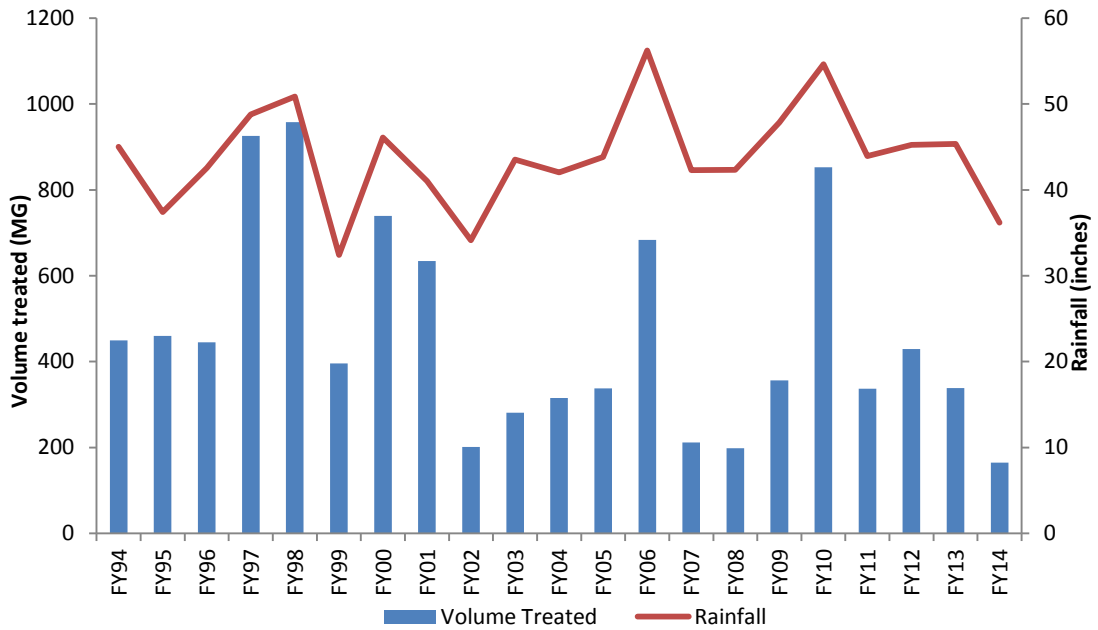
Figure 29. Prison Point CSO Volume Treated Compared to Precipitation, FY94-FY14
