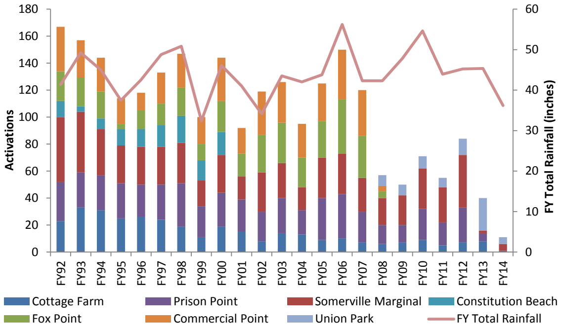
Figure 6. CSO Activations, FY92-FY14
