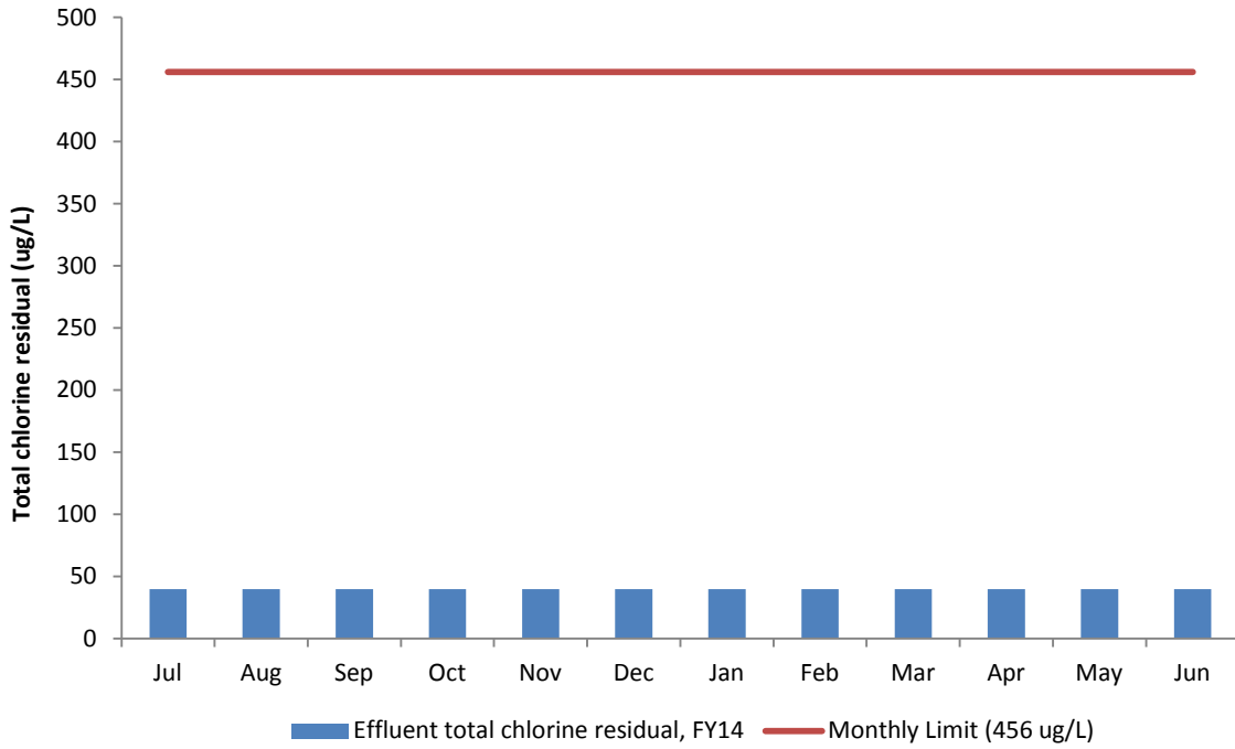
Figure 23. DITP Effluent Total Chlorine Residual (Monthly Average), FY14
