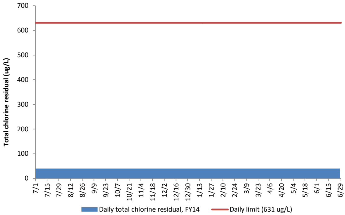
Figure 24. DITP Effluent Total Chlorine Residual (Daily Average), FY14
