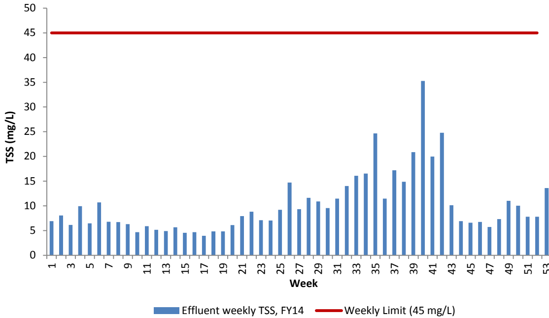
Figure 19. DITP Effluent TSS (Weekly Average), FY14
