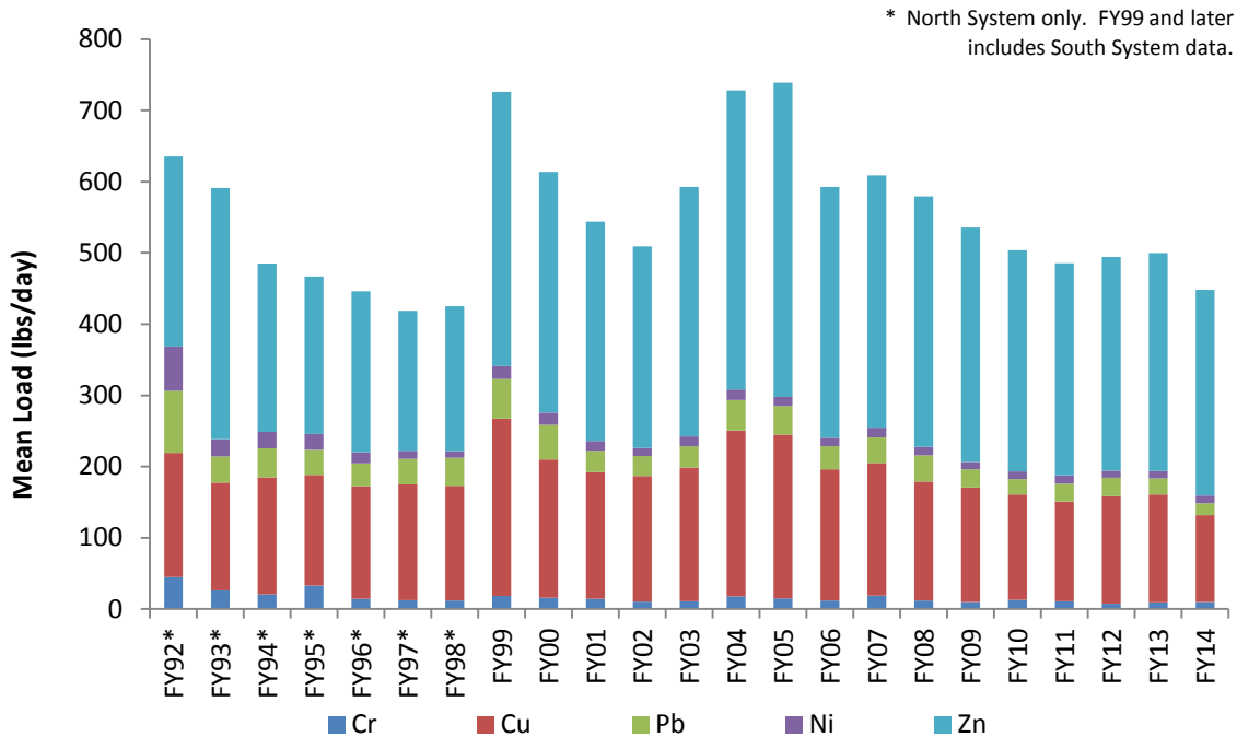
Figure 11. DITP Mean Influent Metals Loadings, FY92-FY14
