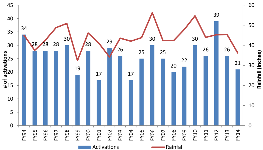
Figure 30. Somerville Marginal CSO Activations Compared to Precipitation, FY94-FY14
