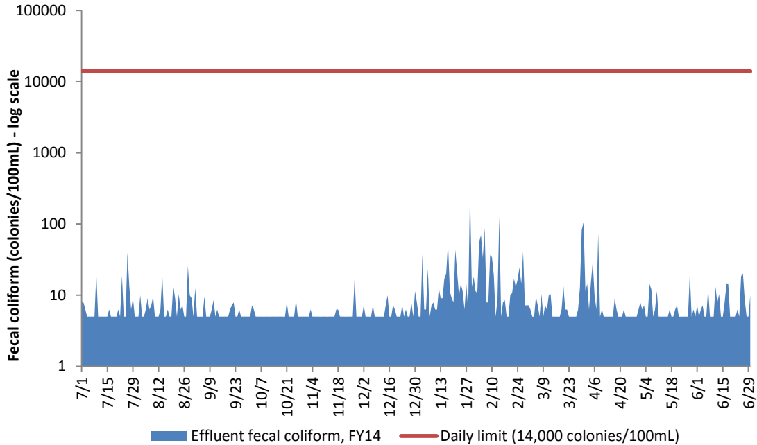
Figure 20. DITP Effluent Fecal Coliform (Daily Geometric Mean), FY14
