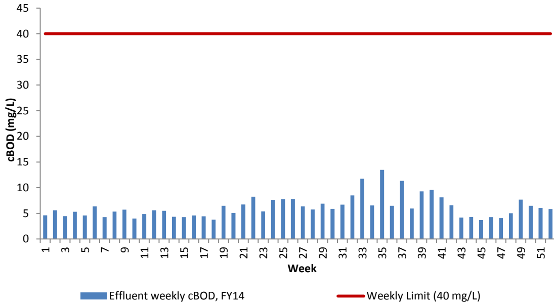
Figure 17. DITP Effluent cBOD (Weekly Average), FY14
