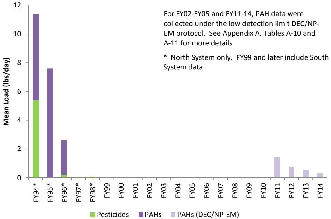
Figure 12b. DITP Mean Influent Organics Loadings, FY94-FY14
