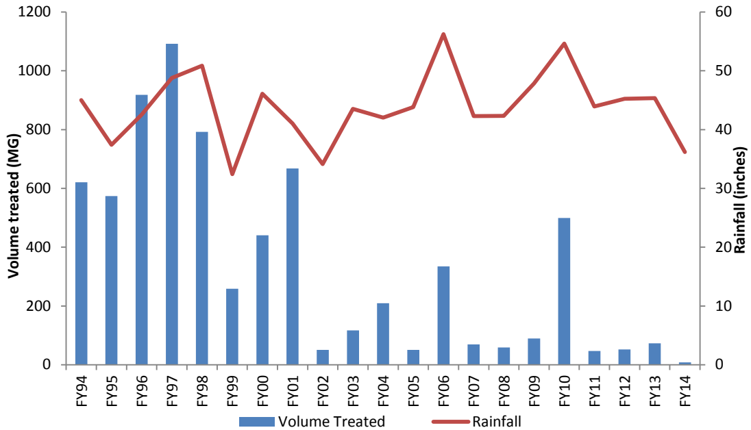
Figure 27. Cottage Farm CSO Volume Treated Compared to Precipitation, FY94-FY14
