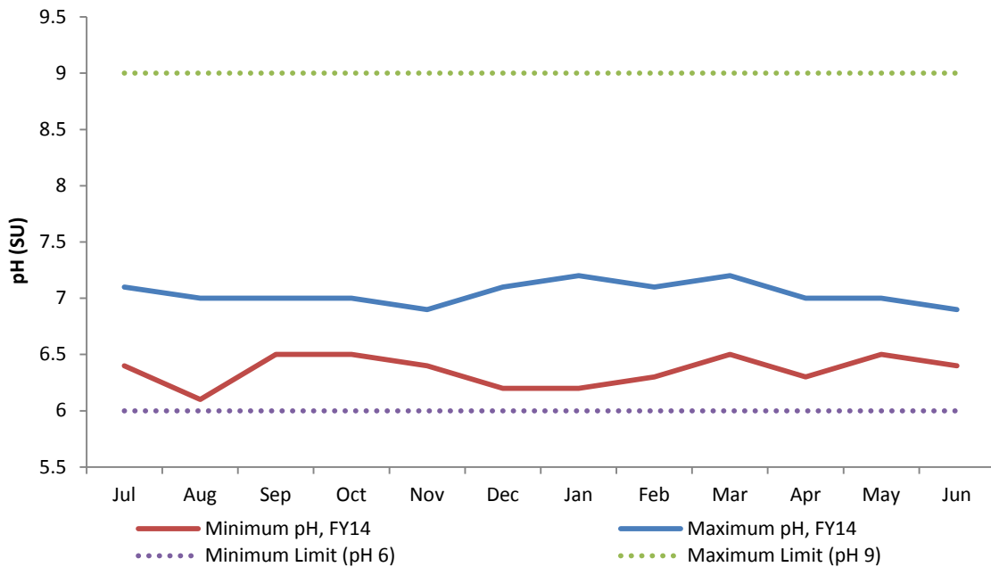
Figure 22. DITP Effluent pH (Monthly Min and Max), FY14
