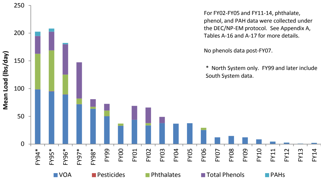
Figure 15. DITP Mean Effluent Organics Loadings, FY94-FY14
