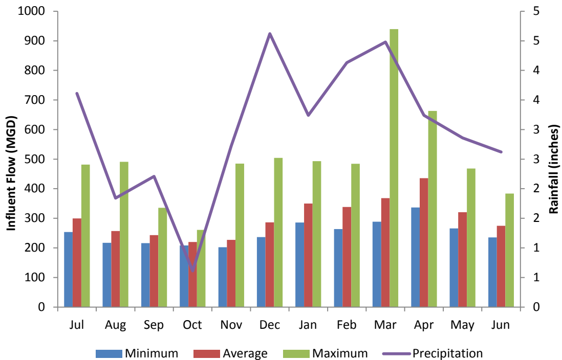
Figure 9. DITP Influent Flow Compared to Precipitation, FY14
