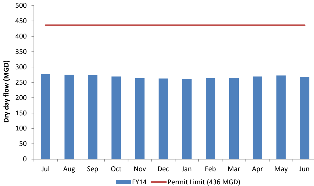
Figure 2. DITP Dry Day Flows, FY14
