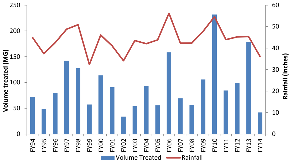
Figure 31. Somerville Marginal CSO Volume Treated Compared to Precipitation, FY94-FY14
