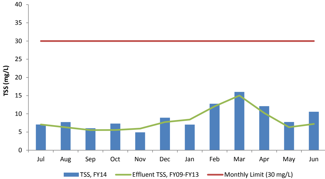
Figure 18. DITP Effluent TSS (Monthly Average), FY14
