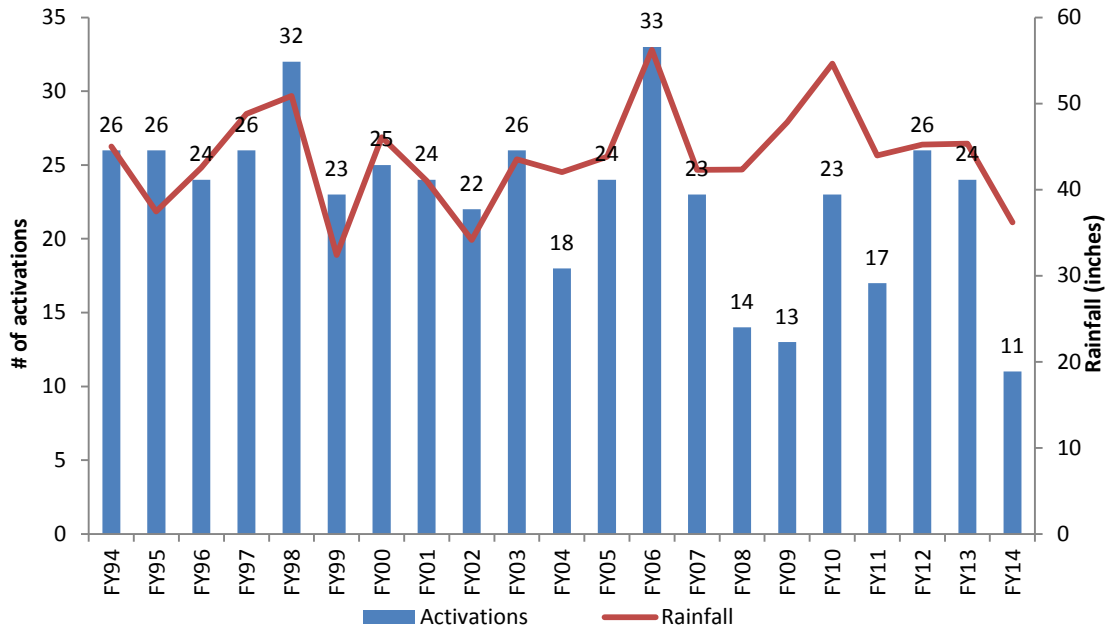
Figure 28. Prison Point CSO Activation Compared to Precipitation, FY94-FY14
