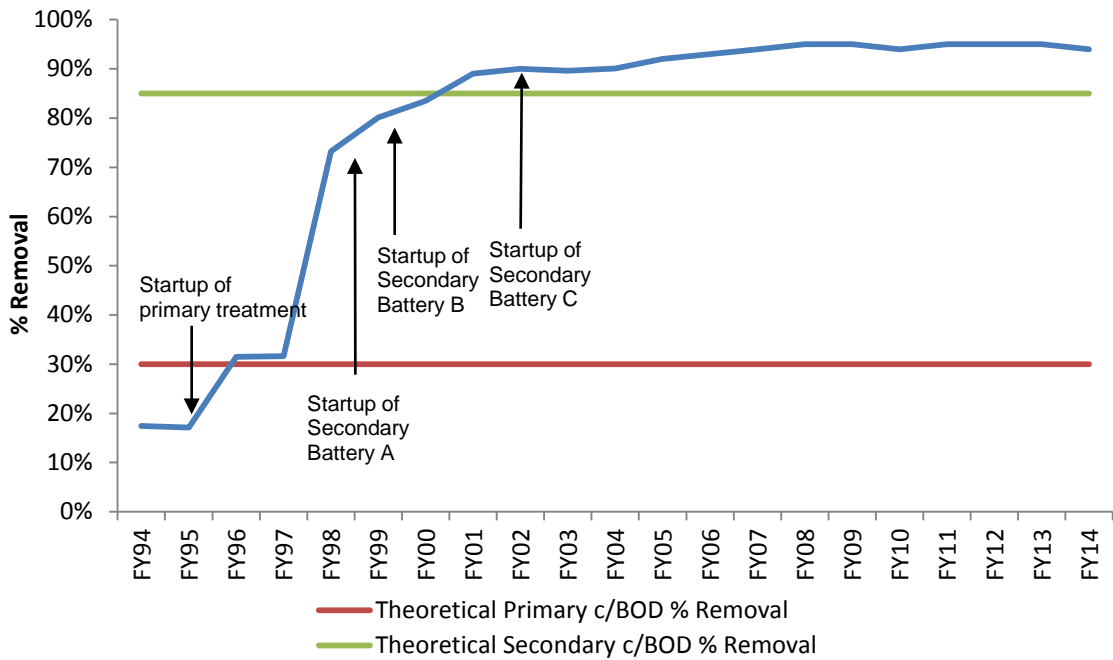
Figure 4. DITP Effluent BOD/cBOD Removal Rate, FY94-FY14
