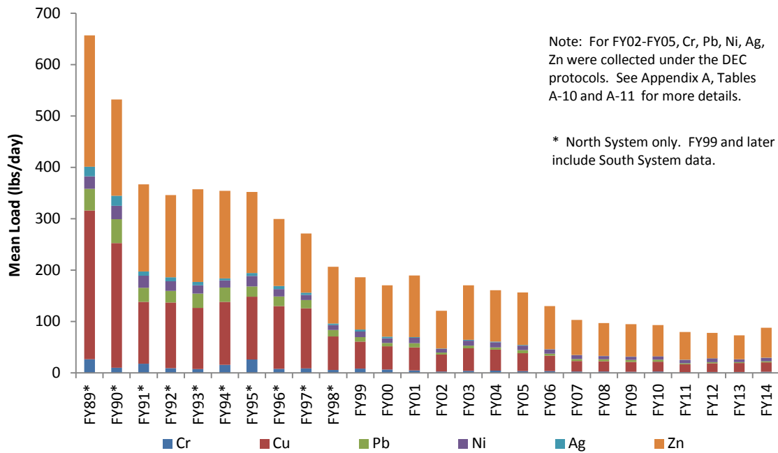
Figure 14. DITP Mean Effluent Metals Loadings, FY89-FY14
