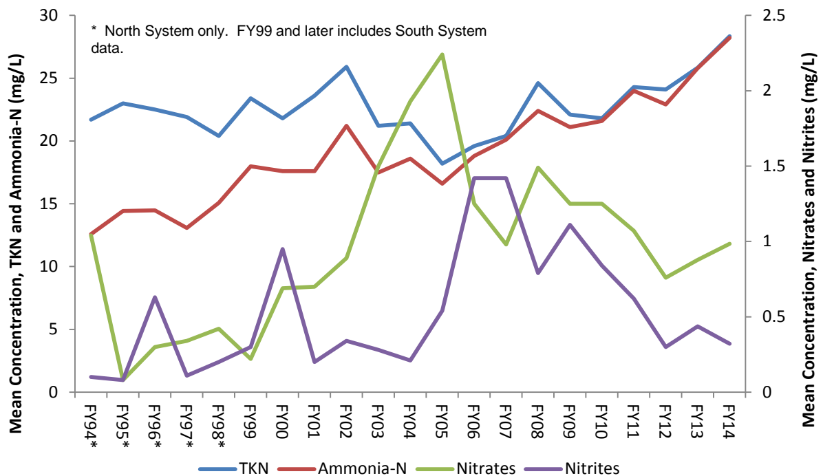
Figure 13. DITP Mean Effluent Nutrients Concentrations, FY94-FY14
