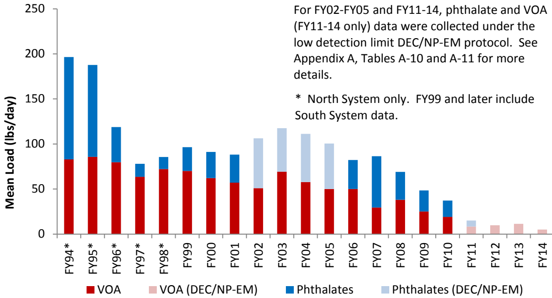
Figure 12a. DITP Mean Influent Organics Loadings, FY94-FY14
