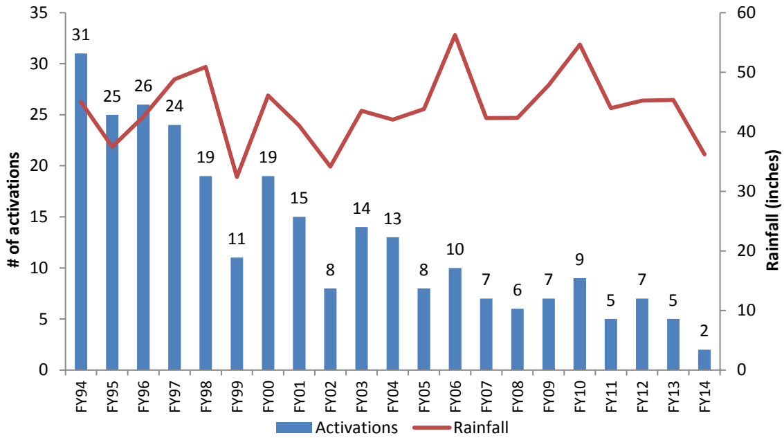
Figure 26. Cottage Farm CSO Activations Compared to Precipitation, FY94-FY14
