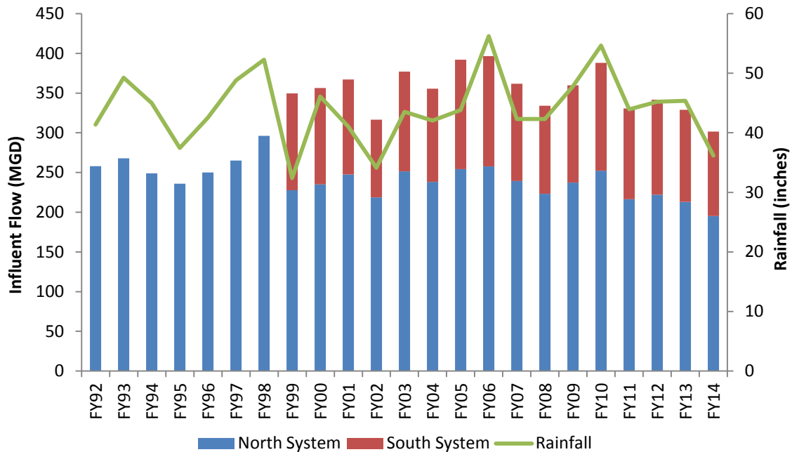
Figure 10. DITP Influent Flow Compared to Precipitation, FY92-FY14
