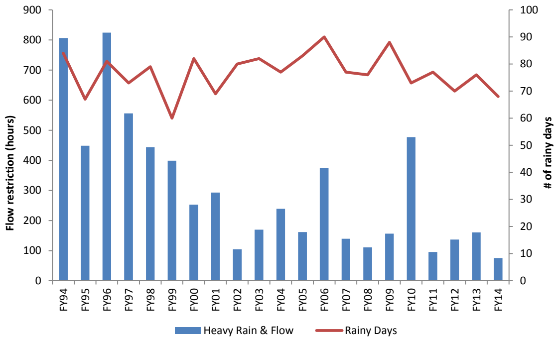
Figure 33. Rain-Related Choking, FY94-FY14
