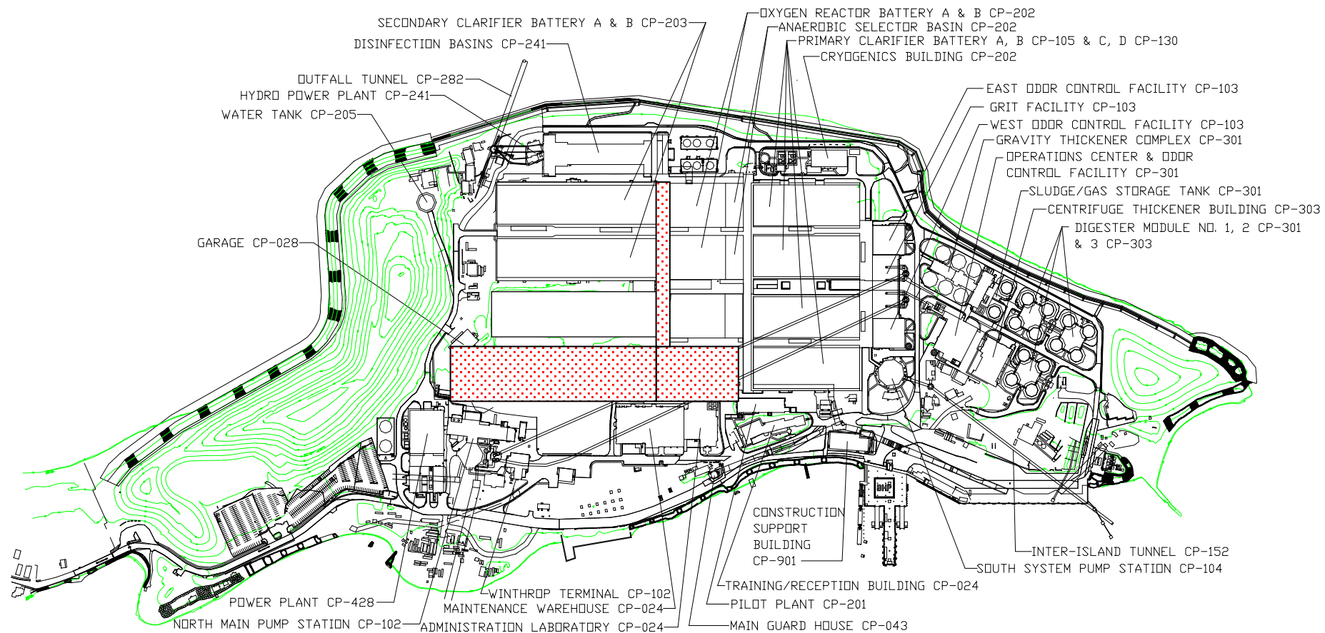
Figure 14. Proposed MBBR nitrification/denitrification layout
