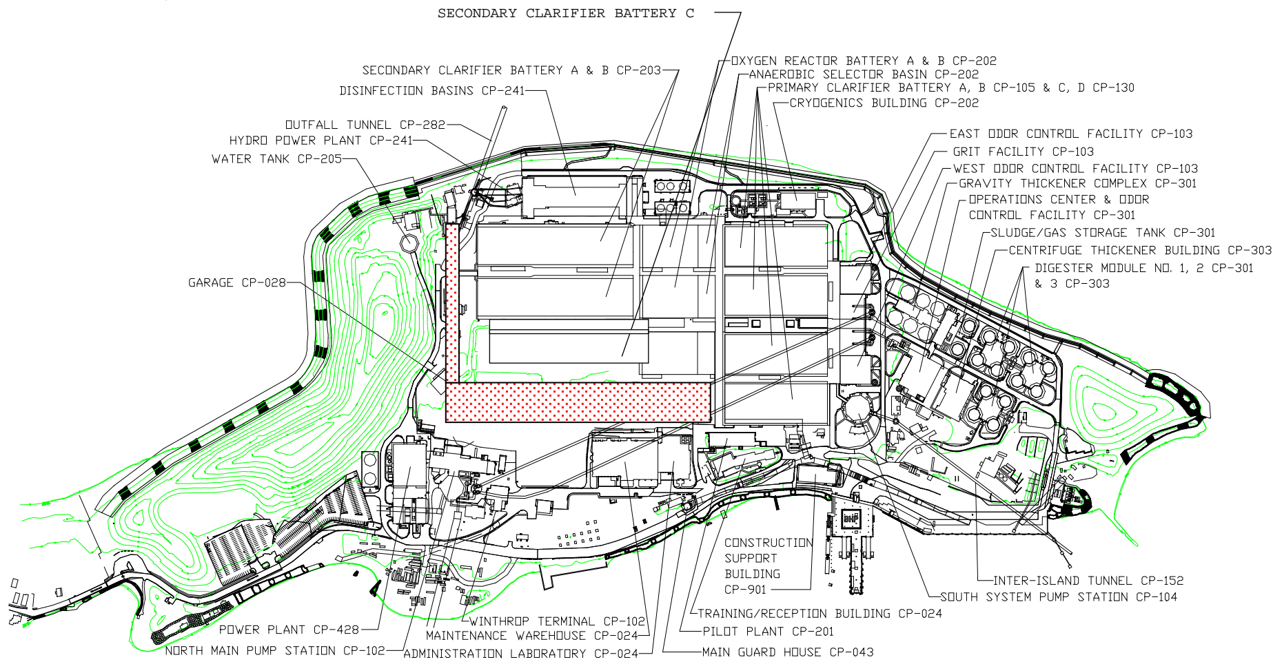
Figure 12. Proposed BAF and SPBR layout
