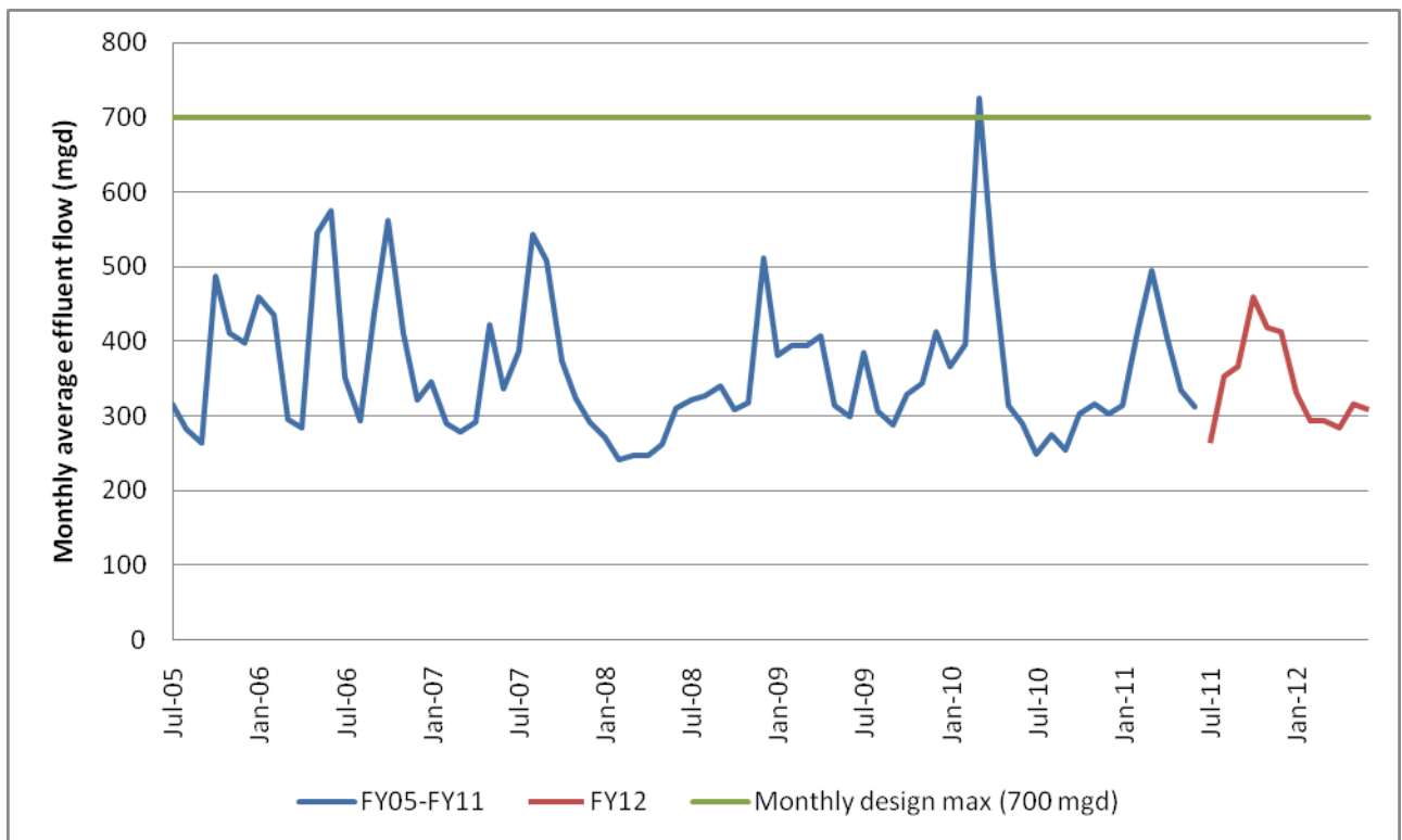
Figure 5. Monthly average flow
