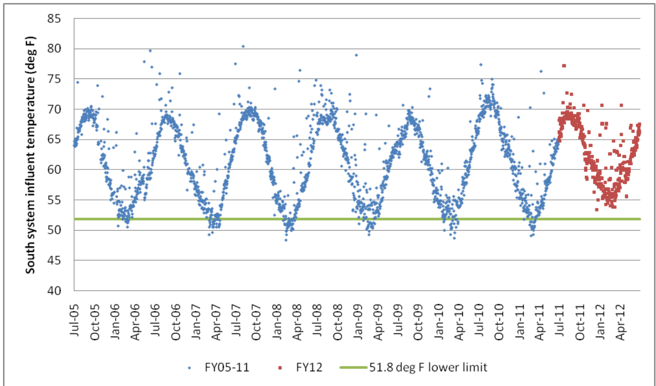
Figure 10. South System influent temperatures
