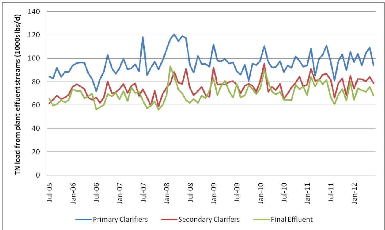
Figure 8. Total nitrogen load from plant effluent streams
