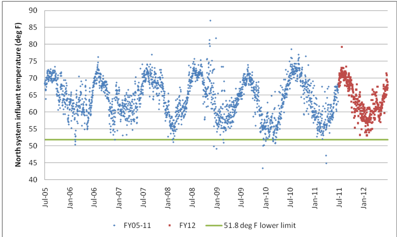
Figure 9. North System influent temperatures
