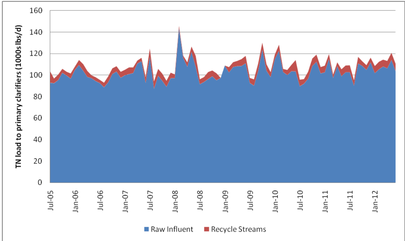
Figure 7. Total nitrogen load to primary clarifiers
