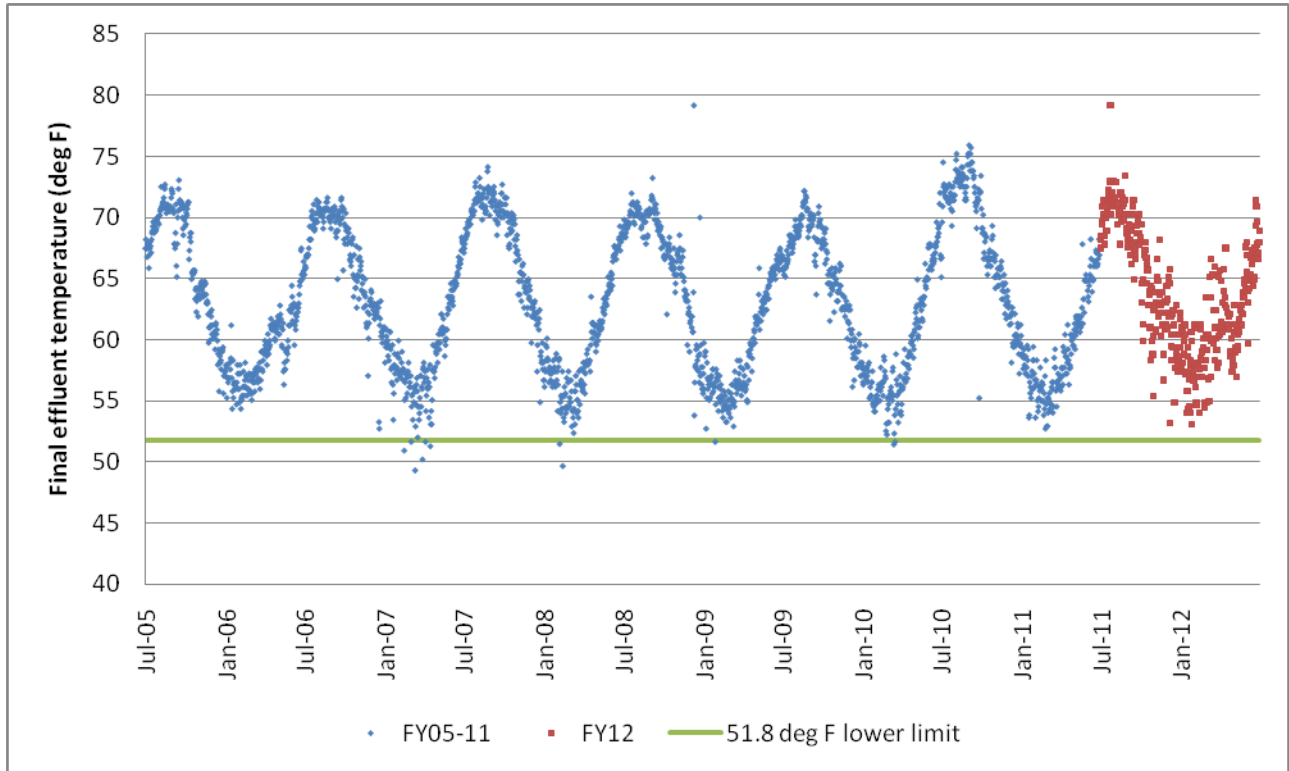
Figure 11. Final effluent temperatures
