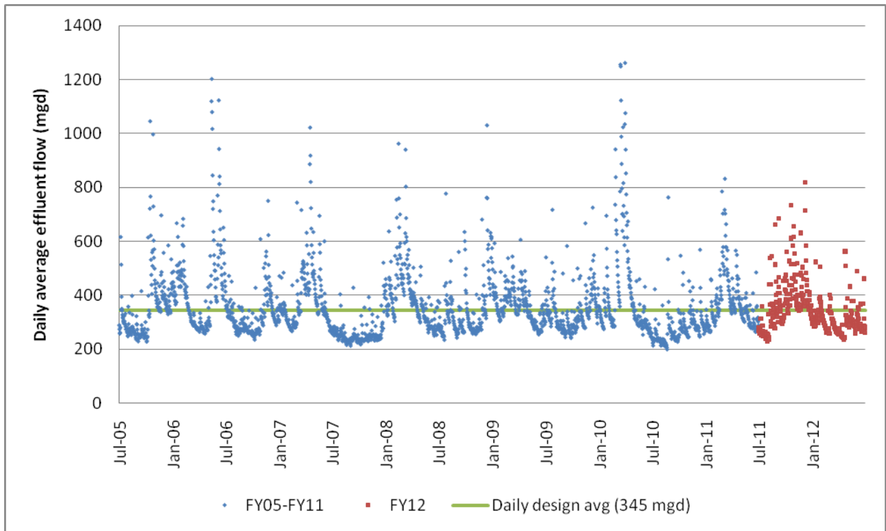
Figure 4. Daily average flow
