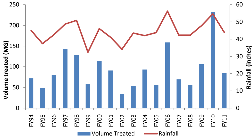
Figure 31. Somerville Marginal CSO Volume Treated Compared to Precipitation, FY94-FY11
