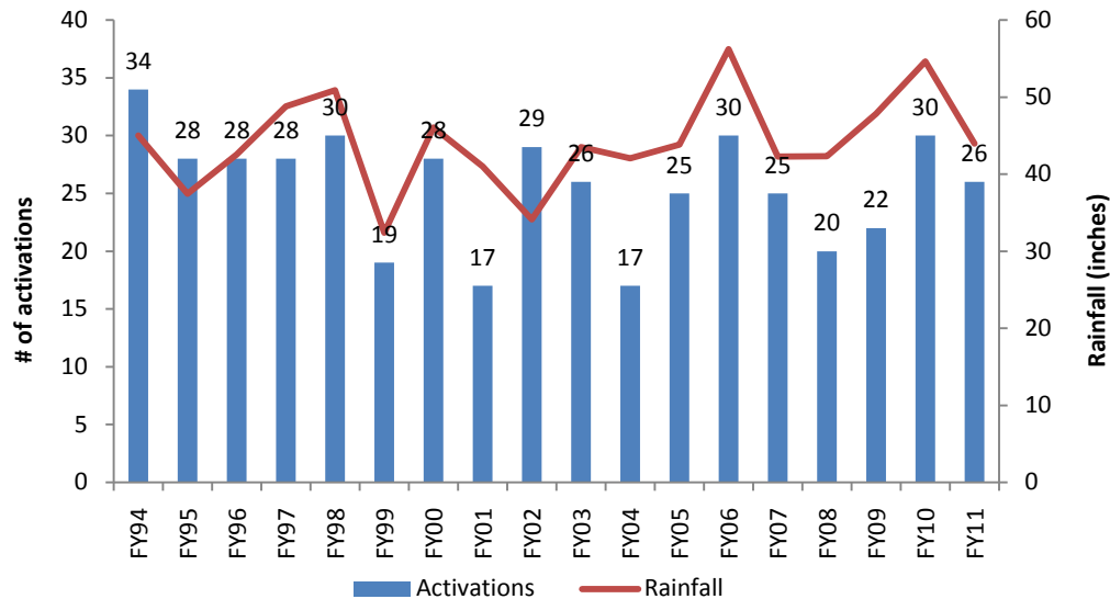
Figure 30. Somerville Marginal CSO Activations Compared to Precipitation, FY94-FY11
