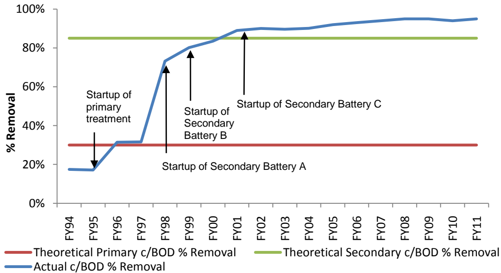
Figure 4. DITP Effluent BOD/cBOD Removal Rate, FY94-FY11
