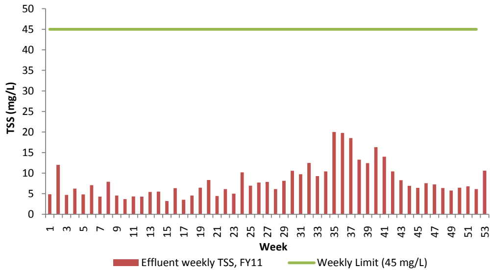
Figure 19. DITP Effluent TSS (Weekly Average), FY11
