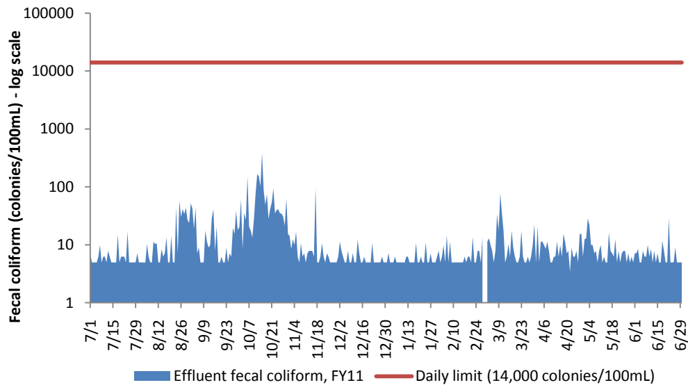
Figure 20. DITP Effluent Fecal Coliform (Daily Geometric Mean), FY11
