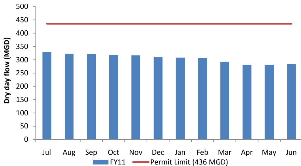
Figure 2. DITP Dry Day Flows, FY11
