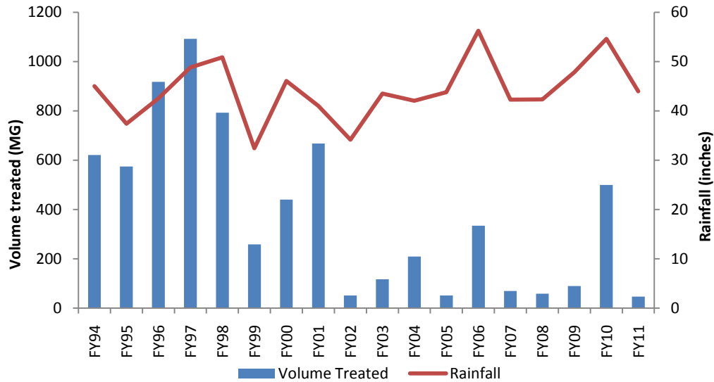
Figure 27. Cottage Farm CSO Volume Treated Compared to Precipitation, FY94-FY11
