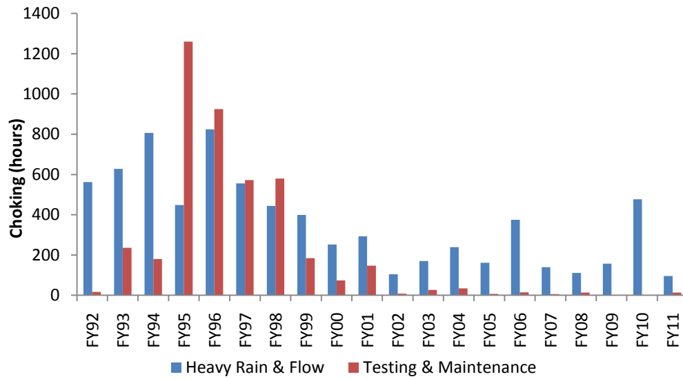
Figure 8. Headworks Choking, FY92-FY11
