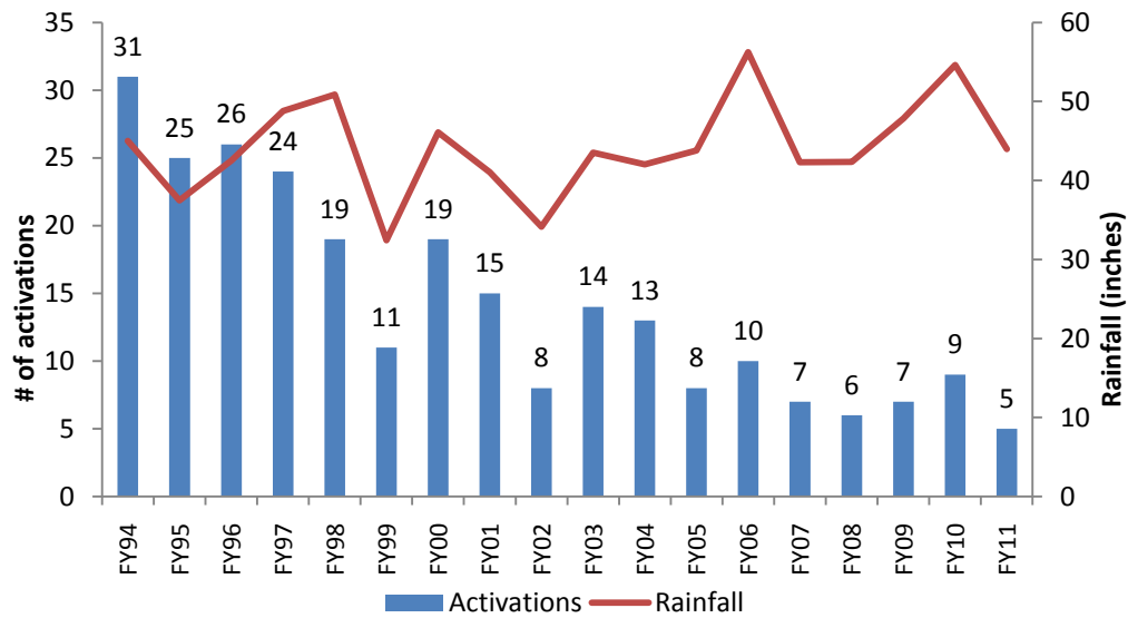
Figure 26. Cottage Farm CSO Activations Compared to Precipitation, FY94-FY11
