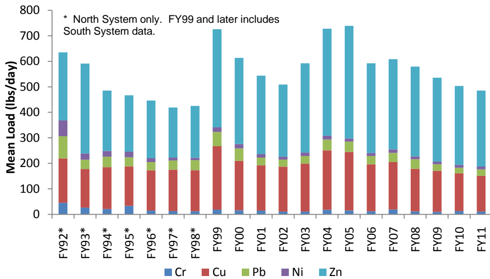
Figure 11. DITP Mean Influent Metals Loadings, FY92-FY11
