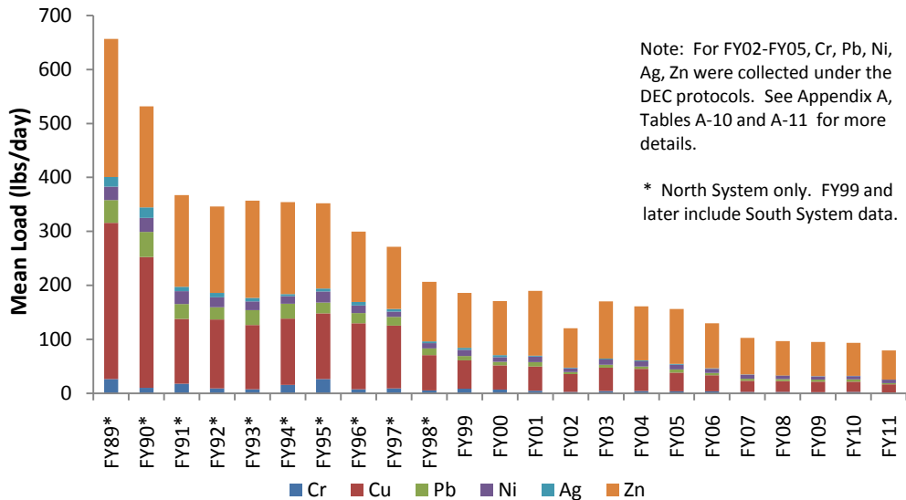
Figure 14. DITP Mean Effluent Metals Loadings, FY89-FY11
