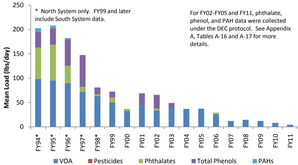
Figure 15. DITP Mean Effluent Organics Loadings, FY94-FY11
