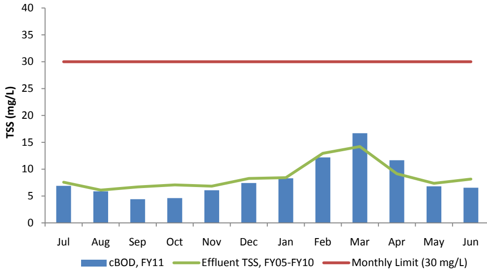
Figure 18. DITP Effluent TSS (Monthly Average), FY11
