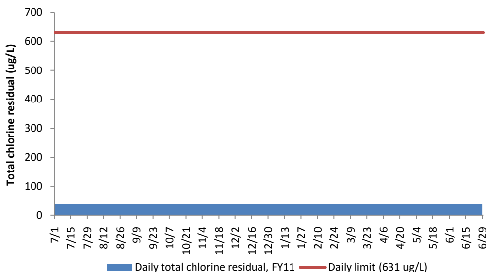
Figure 24. DITP Effluent Total Chlorine Residual (Daily Average), FY11
