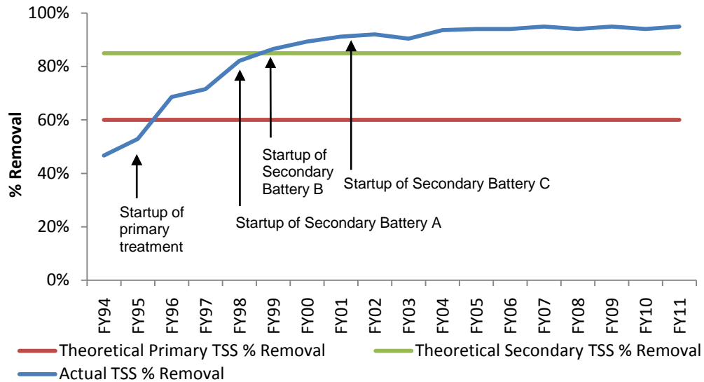
Figure 3. DITP Effluent TSS Removal Rate, FY94-FY11
