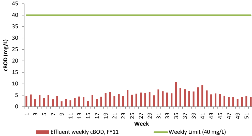
Figure 17. DITP Effluent cBOD (Weekly Average), FY11
