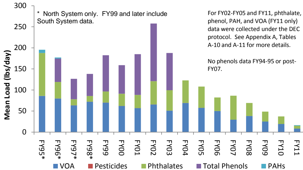
Figure 12. DITP Mean Influent Organics Loadings, FY94-FY11
