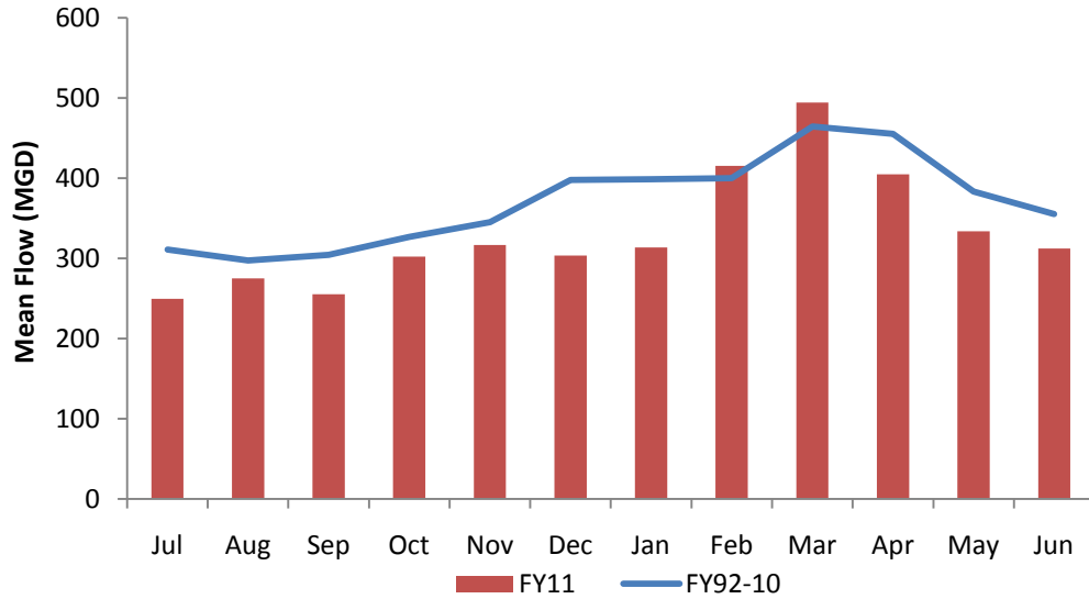
Figure 1. MWRA Flows, FY92-FY11
