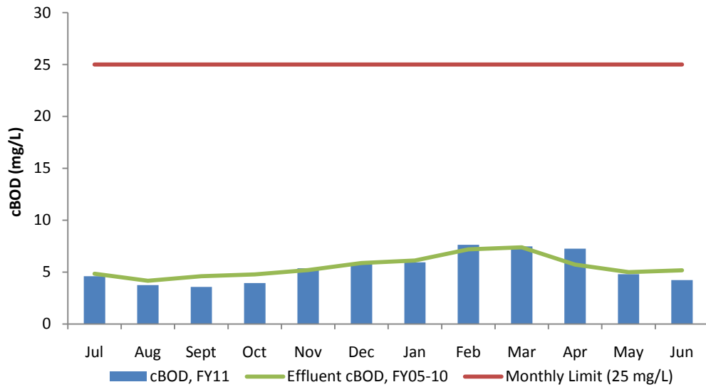
Figure 16. DITP Effluent cBOD (Monthly Average), FY11
