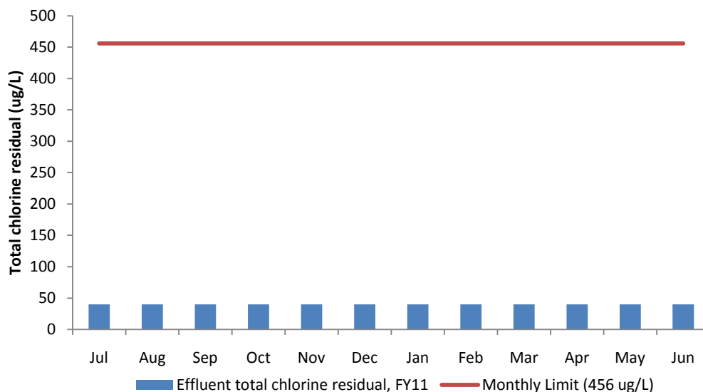
Figure 23. DITP Effluent Total Chlorine Residual (Monthly Average), FY11
