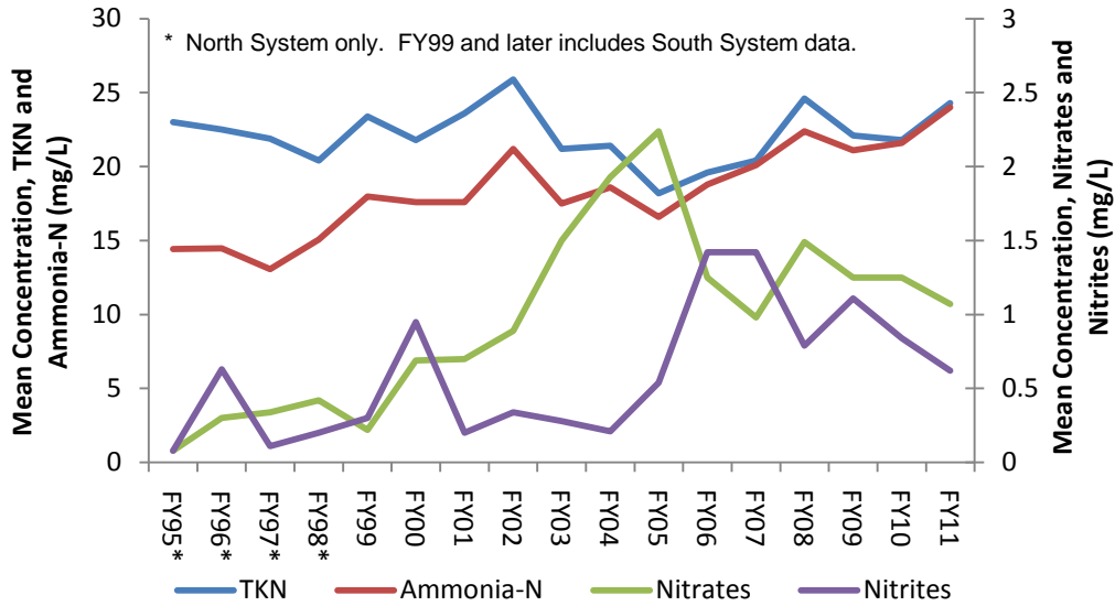
Figure 13. DITP Mean Effluent Nutrients Concentrations, FY94-FY11
