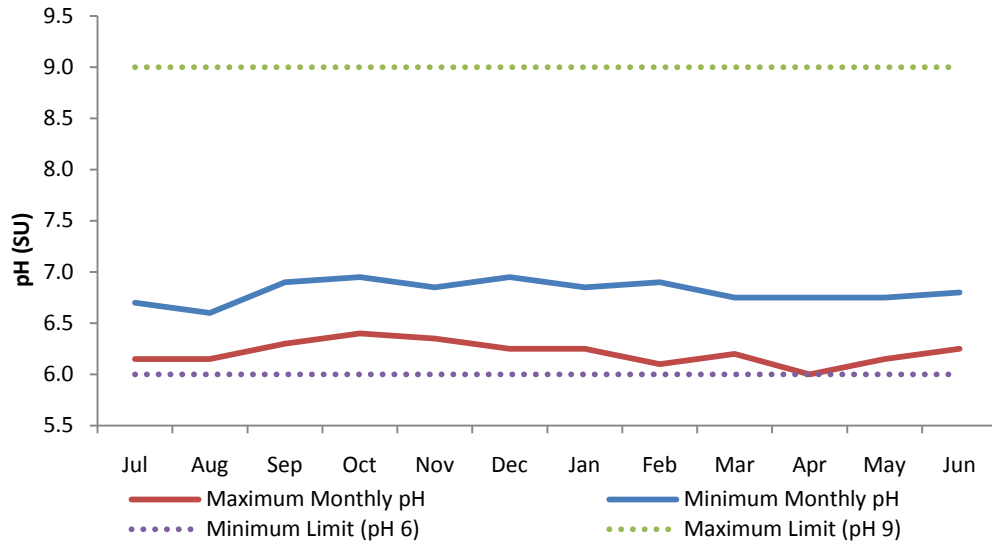
Figure 22. DITP Effluent pH (Monthly Min and Max), FY11
