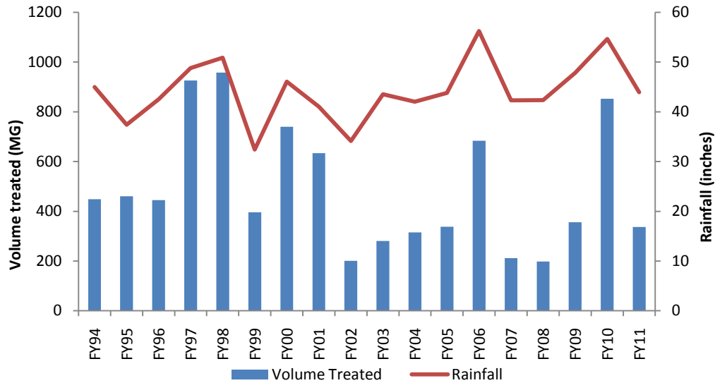
Figure 29. Prison Point CSO Volume Treated Compared to Precipitation, FY94-FY11
