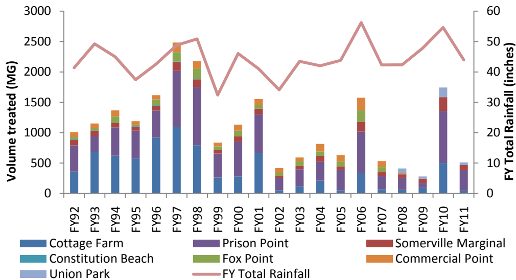
Figure 7. CSO Volume Treated, FY92-FY11
