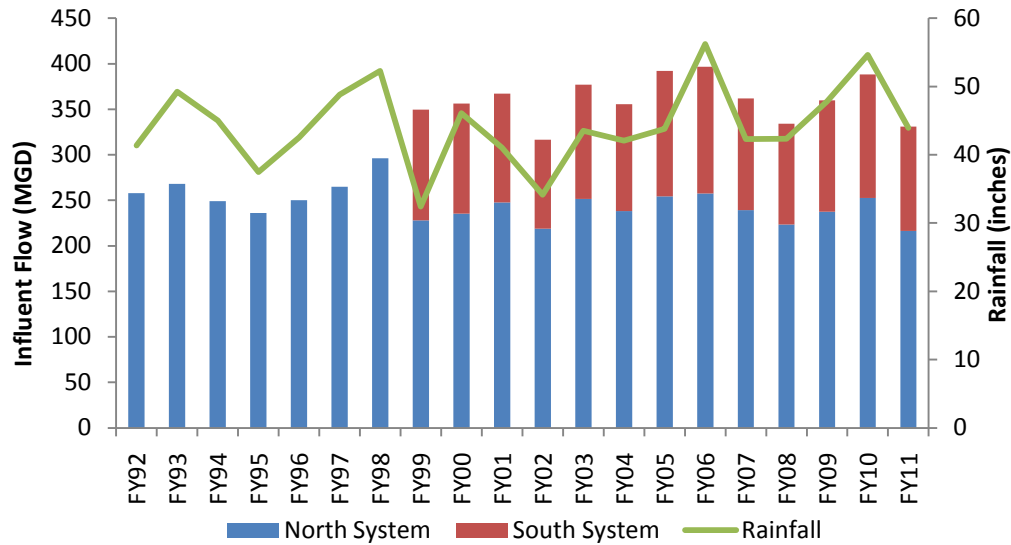
Figure 10. DITP Influent Flow Compared to Precipitation, FY92-FY11
