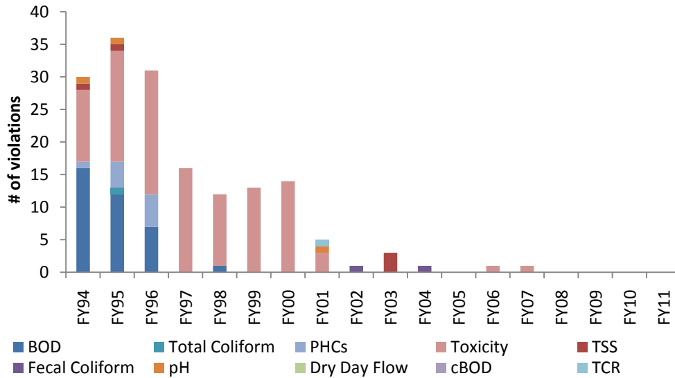
Figure 5. NPDES Violations at DITP, FY94-FY11
