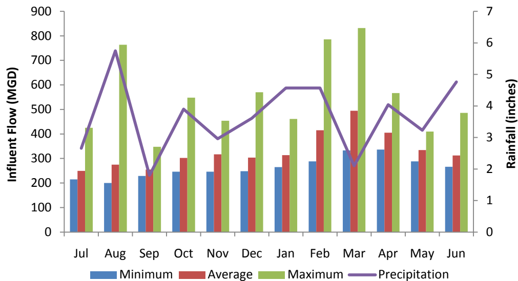
Figure 9. DITP Influent Flow Compared to Precipitation, FY11
