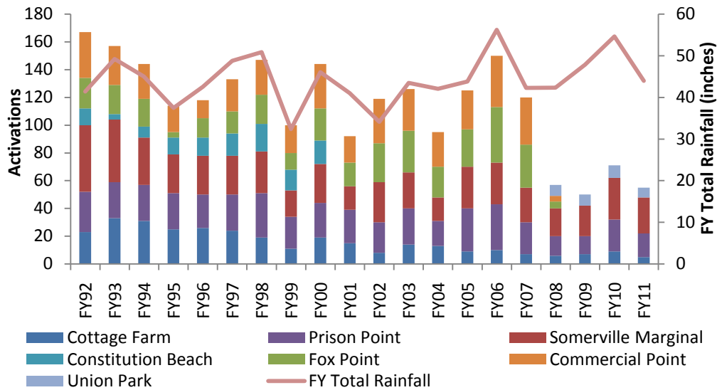
Figure 6. CSO Activations, FY92-FY11
