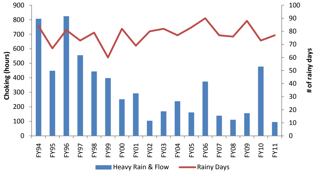
Figure 33. Rain-Related Choking, FY94-FY11
