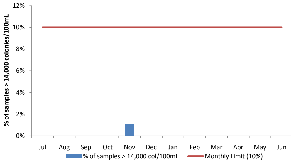
Figure 21. DITP Effluent Fecal Coliform (High Sample Counts), FY11
