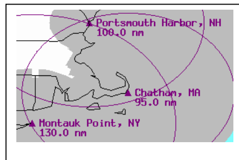
Figure B-5. dGPS Master Stations Coverage
