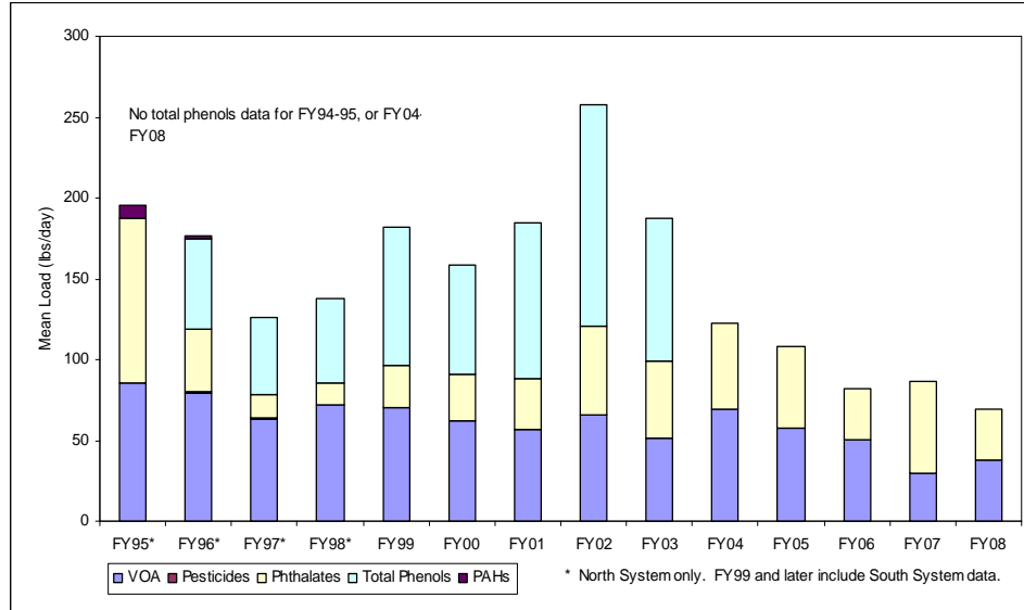
Figure 12. DITP Mean Influent Organics Loadings, FY94-FY08
