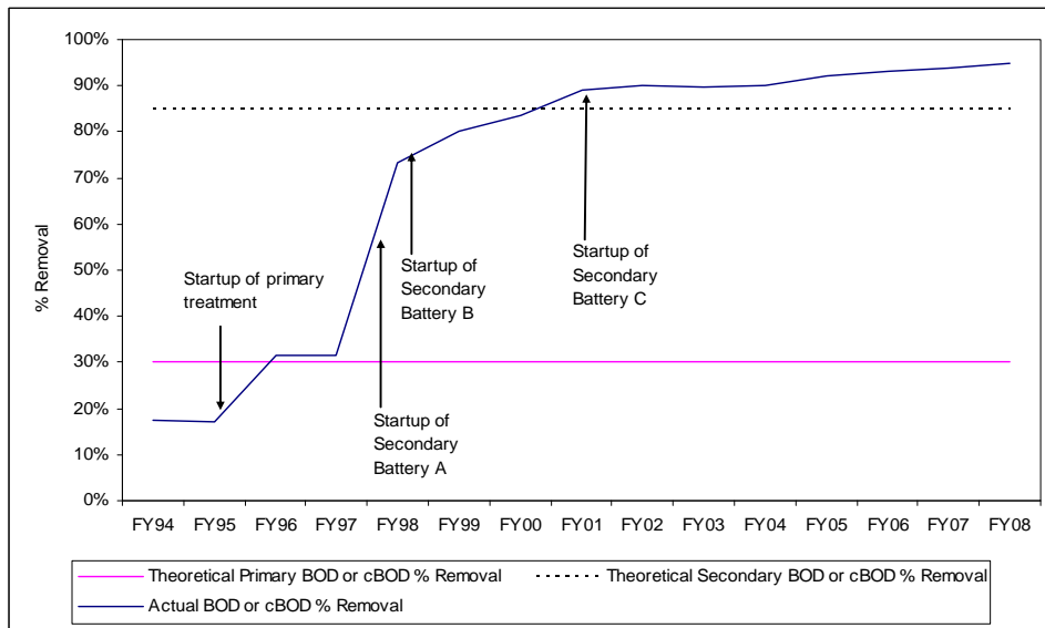
Figure 4. DITP Effluent BOD/cBOD Removal Rate, FY94-FY08
