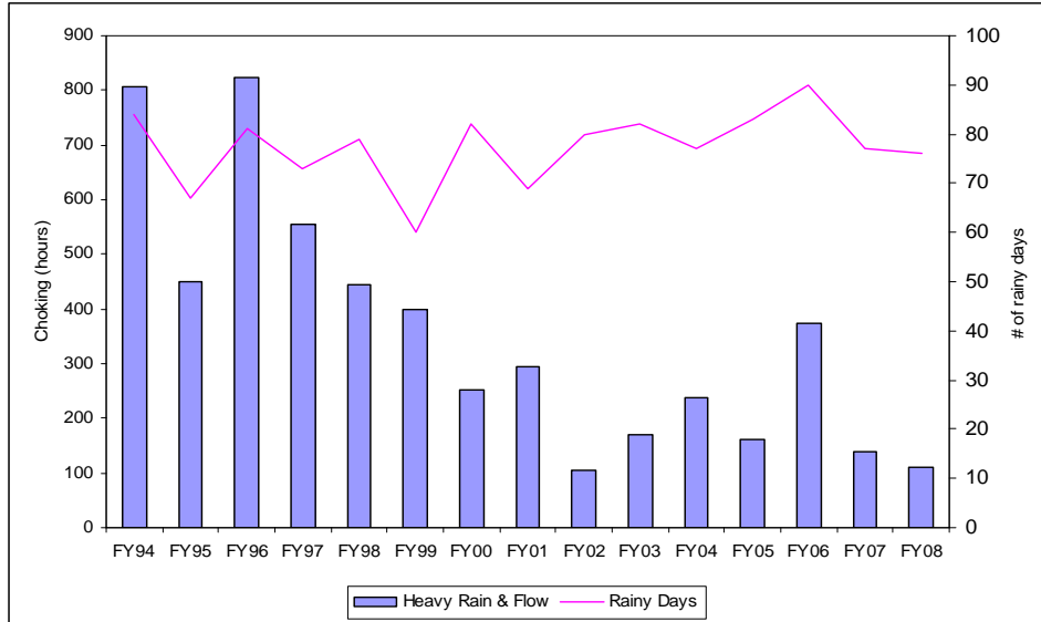
Figure 37. Rain-Related Choking, FY94-FY08
