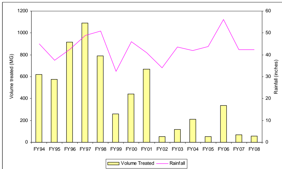
Figure 27. Cottage Farm CSO Volume Treated Compared to Precipitation, FY94-FY08
