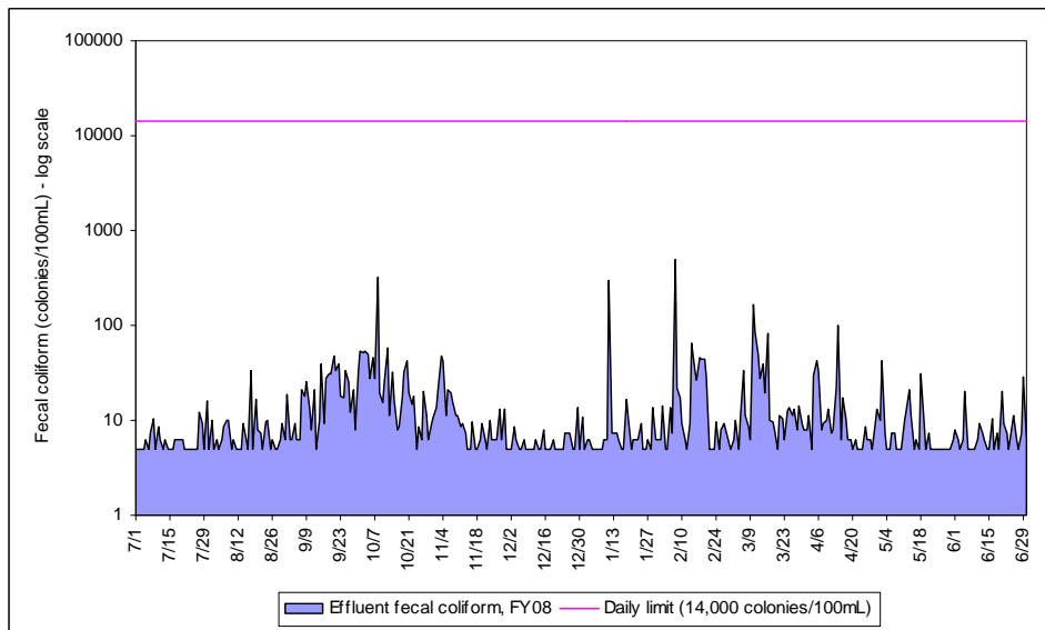
Figure 20. DITP Effluent Fecal Coliform (Daily Geometric Mean), FY08
