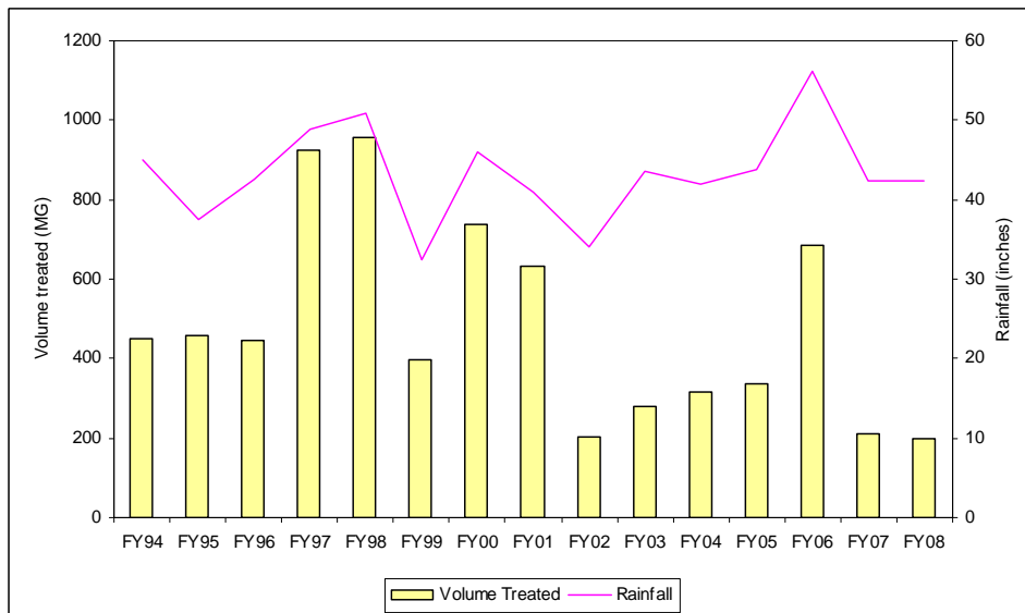
Figure 29. Prison Point CSO Volume Treated Compared to Precipitation, FY94-FY08
