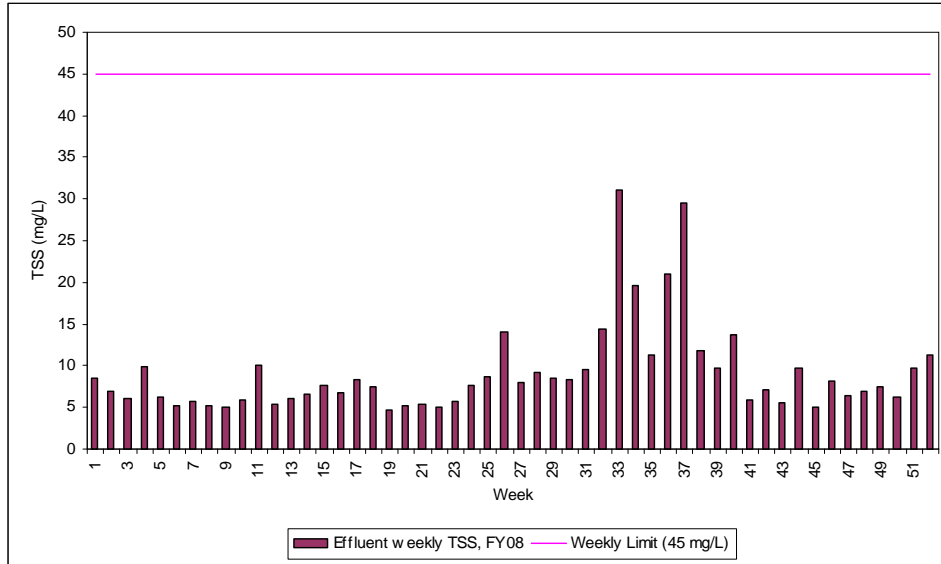
Figure 19. DITP Effluent TSS (Weekly Average), FY08
