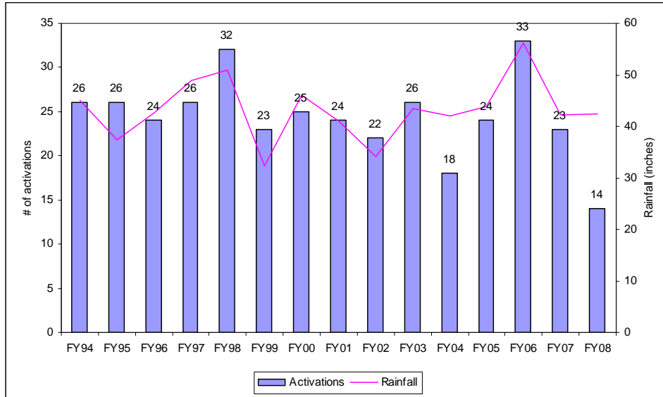
Figure 28. Prison Point CSO Activation Compared to Precipitation, FY94-FY08
