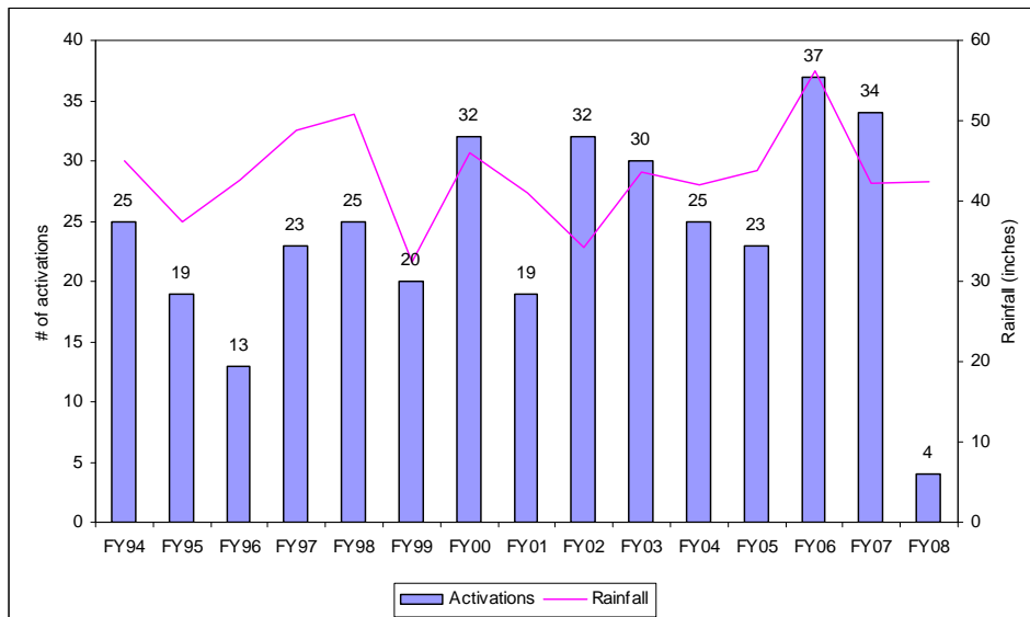
Figure 34. Commercial Point CSO Activation Compared to Precipitation, FY94-FY08
