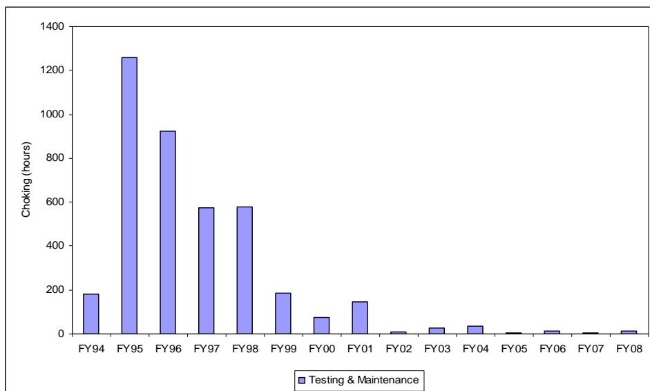
Figure 38. Testing and Maintenance-Related Choking, FY94-FY08
