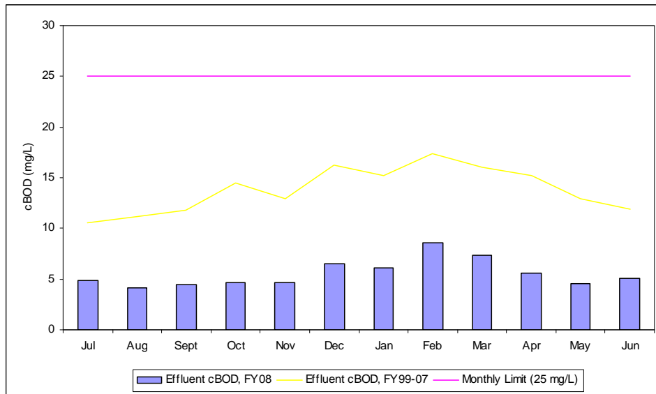
Figure 16. DITP Effluent cBOD (Monthly Average), FY08
