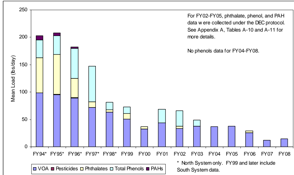
Figure 15. DITP Mean Effluent Organics Loadings, FY94-FY08
