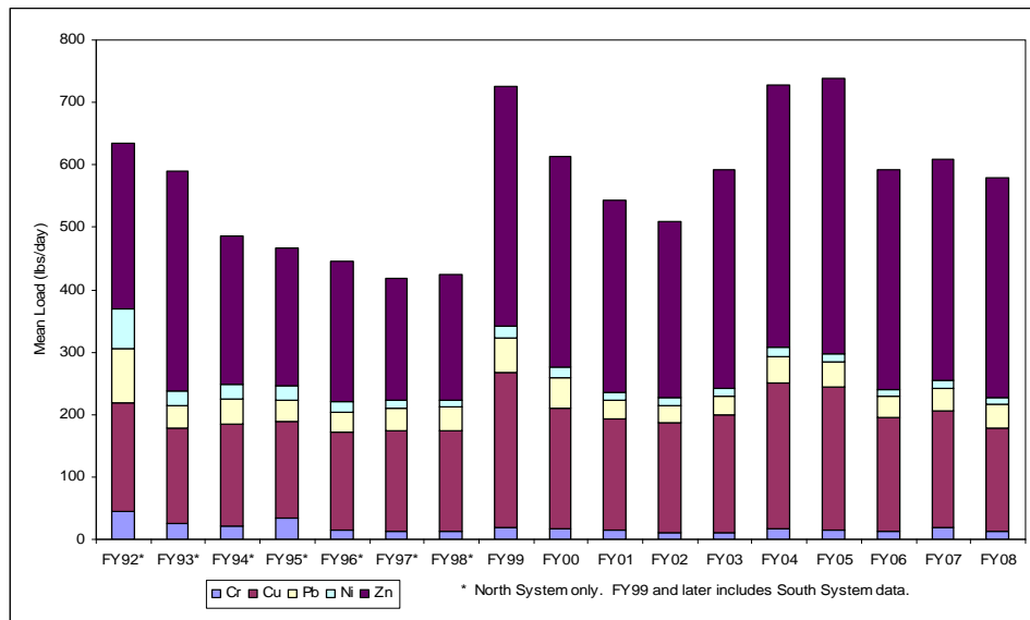
Figure 11. DITP Mean Influent Metals Loadings, FY92-FY08
