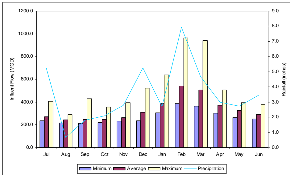
Figure 9. DITP Influent Flow Compared to Precipitation, FY08
