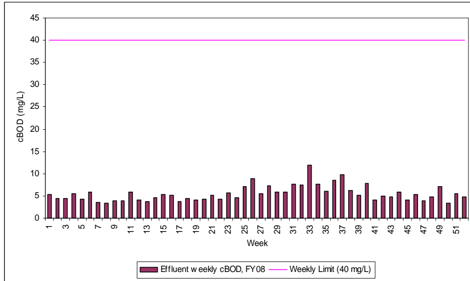
Figure 17. DITP Effluent cBOD (Weekly Average), FY08
