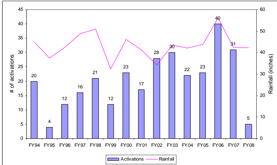
Figure 32. Fox Point CSO Activations Compared to Precipitation, FY94-FY08
