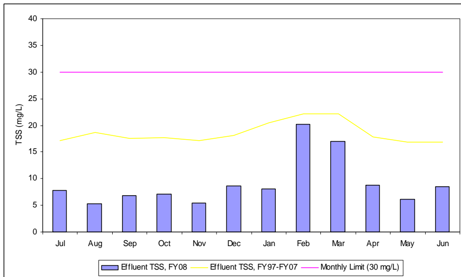
Figure 18. DITP Effluent TSS (Monthly Average), FY08
