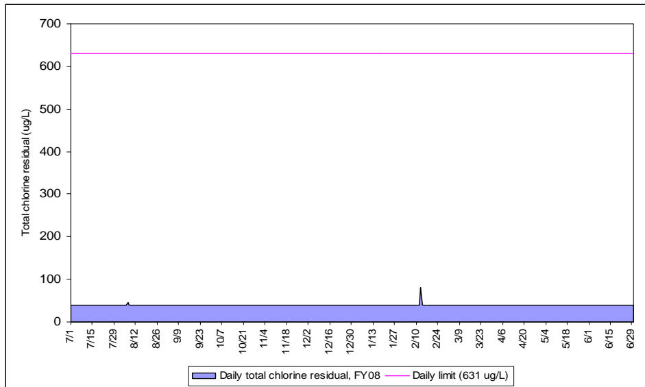
Figure 24. DITP Effluent Total Chlorine Residual (Daily Average), FY08
