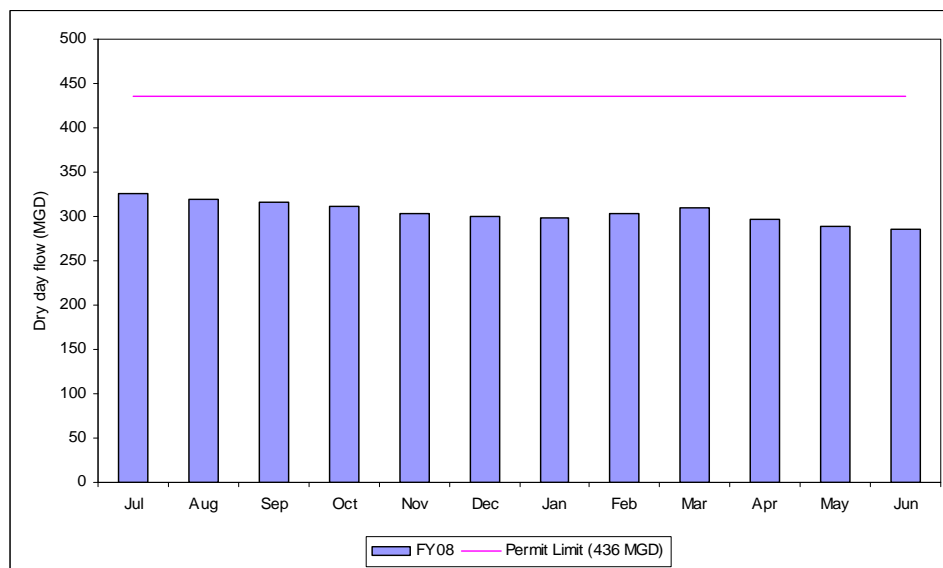
Figure 2. DITP Dry Day Flows, FY08
