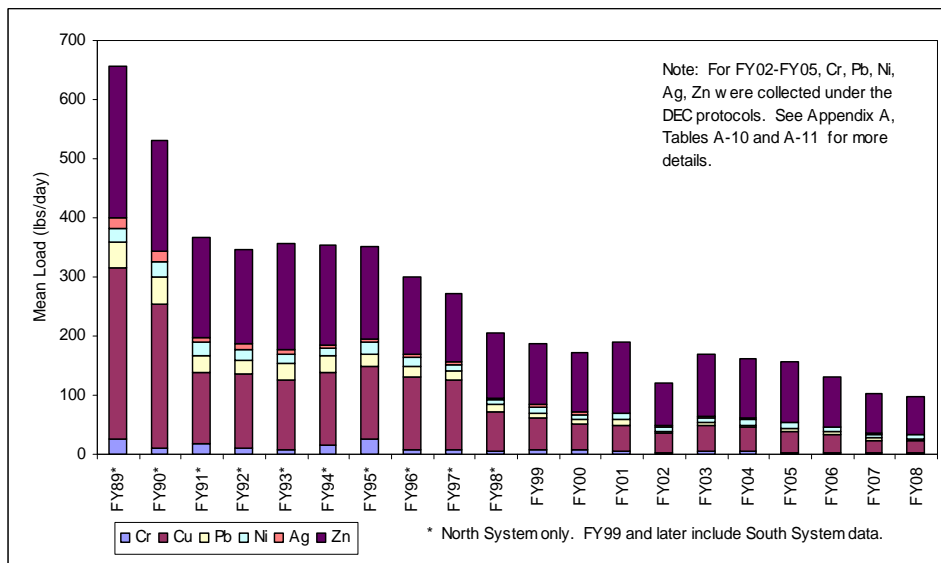
Figure 14. DITP Mean Effluent Metals Loadings, FY89-FY08
