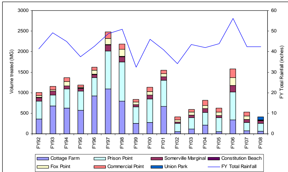
Figure 7. CSO Volume Treated, FY92-FY08
