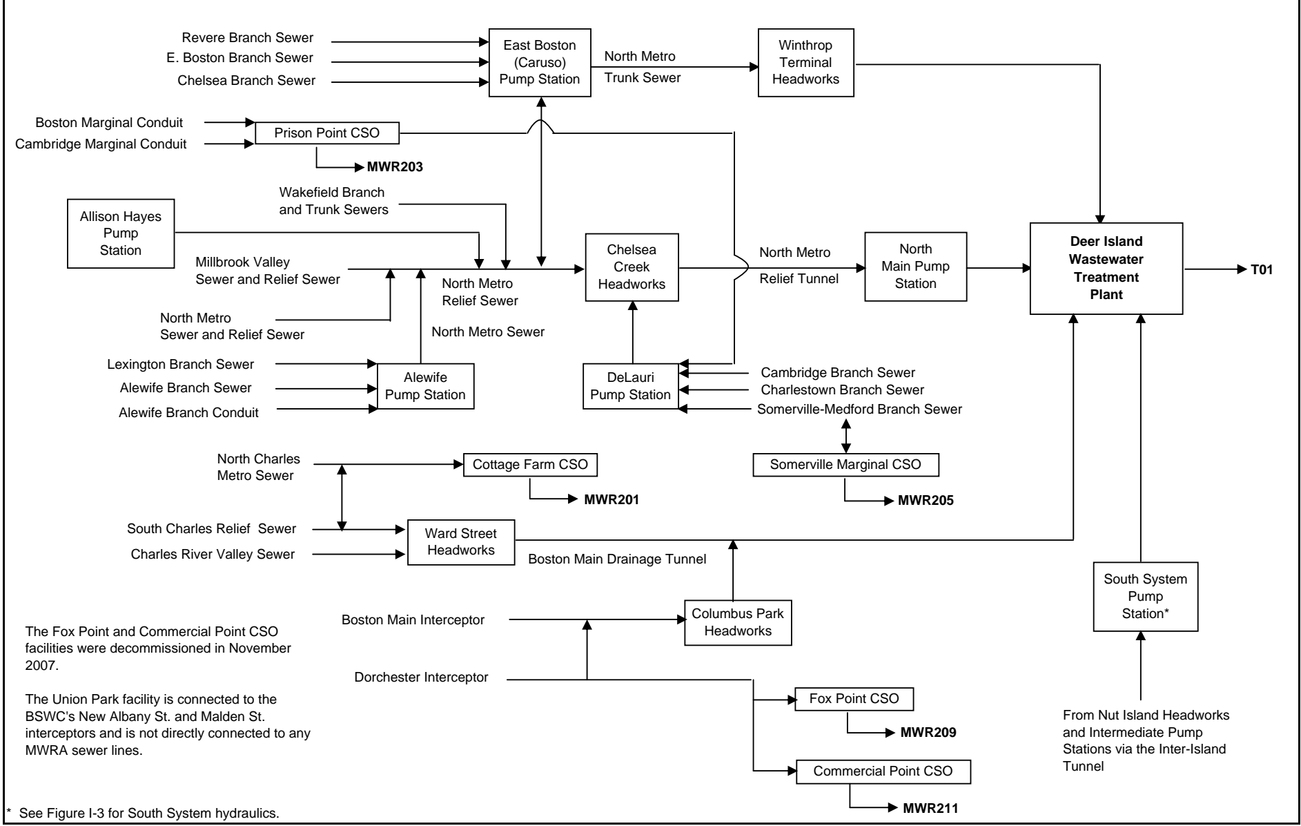
Figure I-1. North System Pump Stations, Headworks, CSOs and Tunnel Hydraulic Schematic
