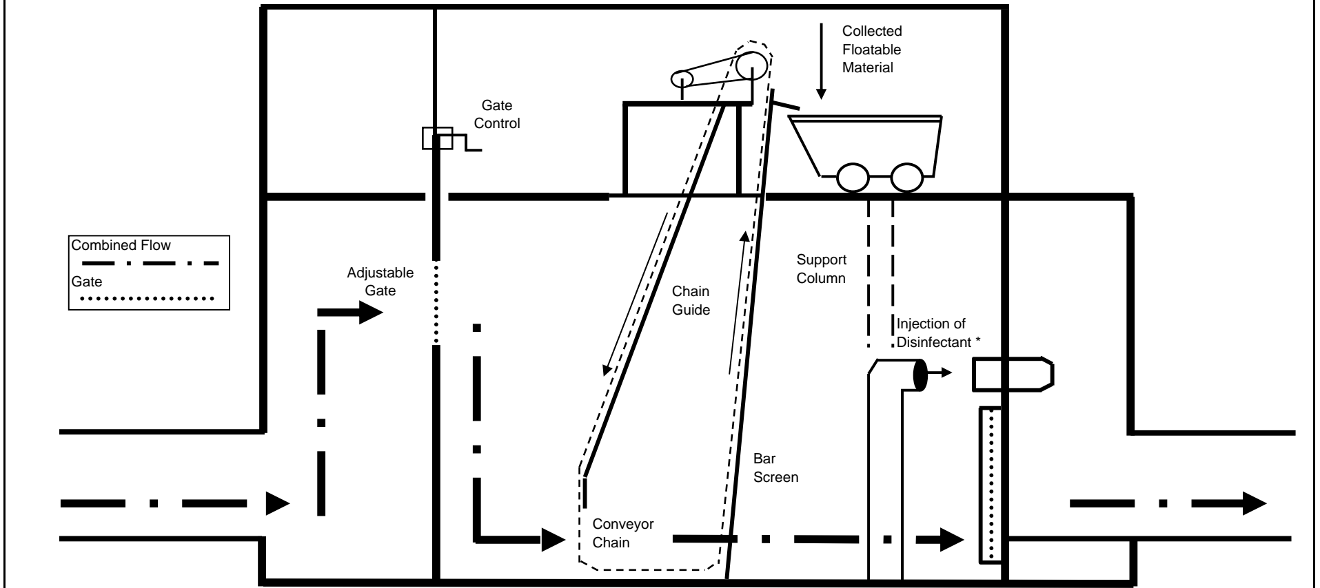
Figure I-2. Typical Gravity Combined Sewer Overflow Treatment Facility
