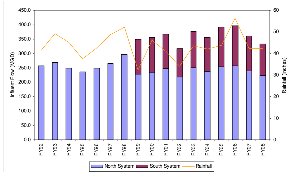
Figure 10. DITP Influent Flow Compared to Precipitation, FY92-FY08
