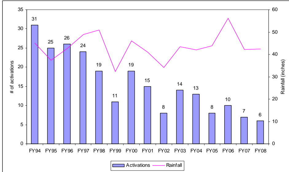
Figure 26. Cottage Farm CSO Activations Compared to Precipitation, FY94-FY08
