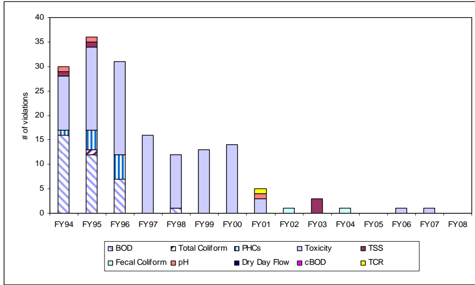
Figure 5. NPDES Violations at DITP, FY94-FY08
