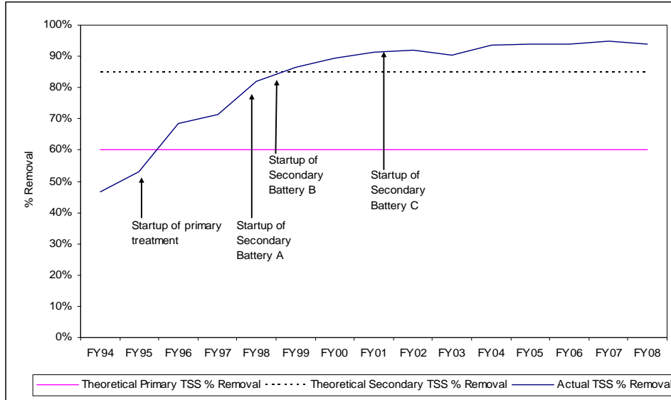
Figure 3. DITP Effluent TSS Removal Rate, FY94-FY08
