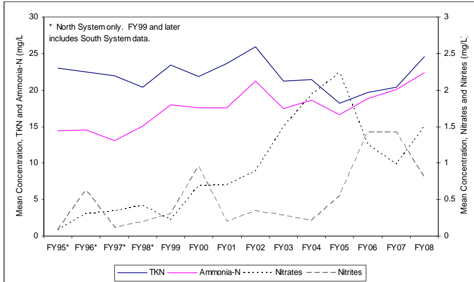
Figure 13. DITP Mean Effluent Nutrients Concentrations, FY94-FY08
