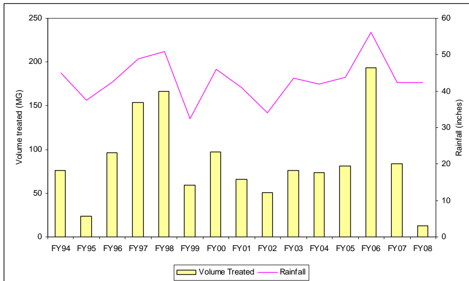
Figure 33. Fox Point CSO Volume Treated Compared to Precipitation, FY94-FY08
