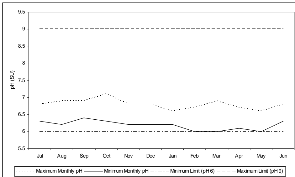
Figure 22. DITP Effluent pH (Monthly Min and Max), FY08
