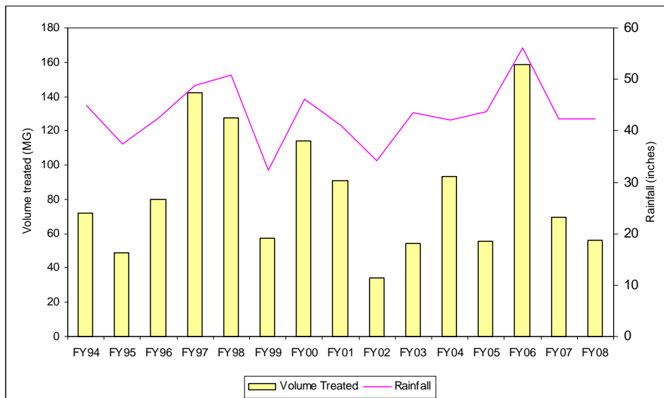
Figure 31. Somerville Marginal CSO Volume Treated Compared to Precipitation, FY94-FY08
