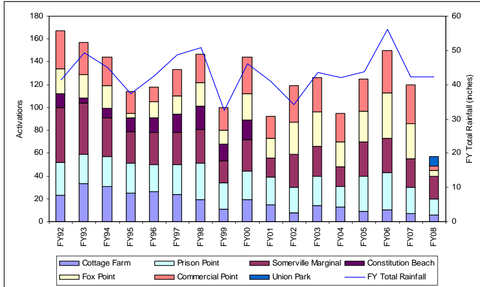
Figure 6. CSO Activations, FY92-FY08
