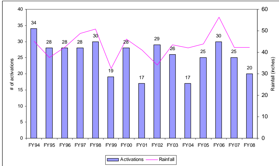
Figure 30. Somerville Marginal CSO Activations Compared to Precipitation, FY94-FY08
