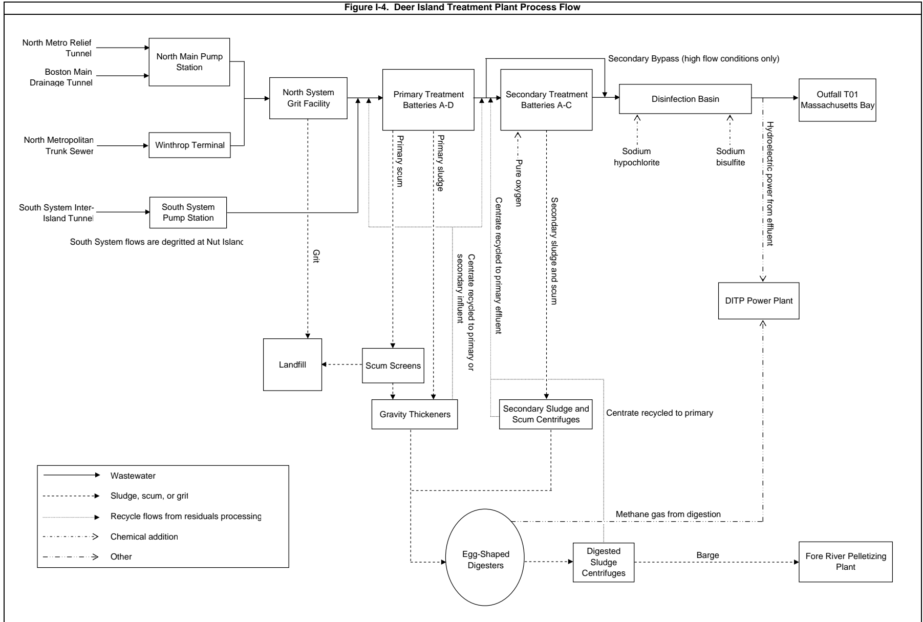
Figure I-4. Deer Island Treatment Plant Process Flow
