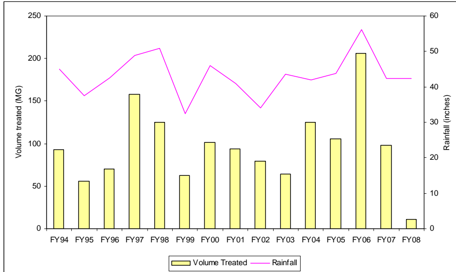
Figure 35. Commercial Point CSO Volume Treated Compared to Precipitation, FY94-FY08
