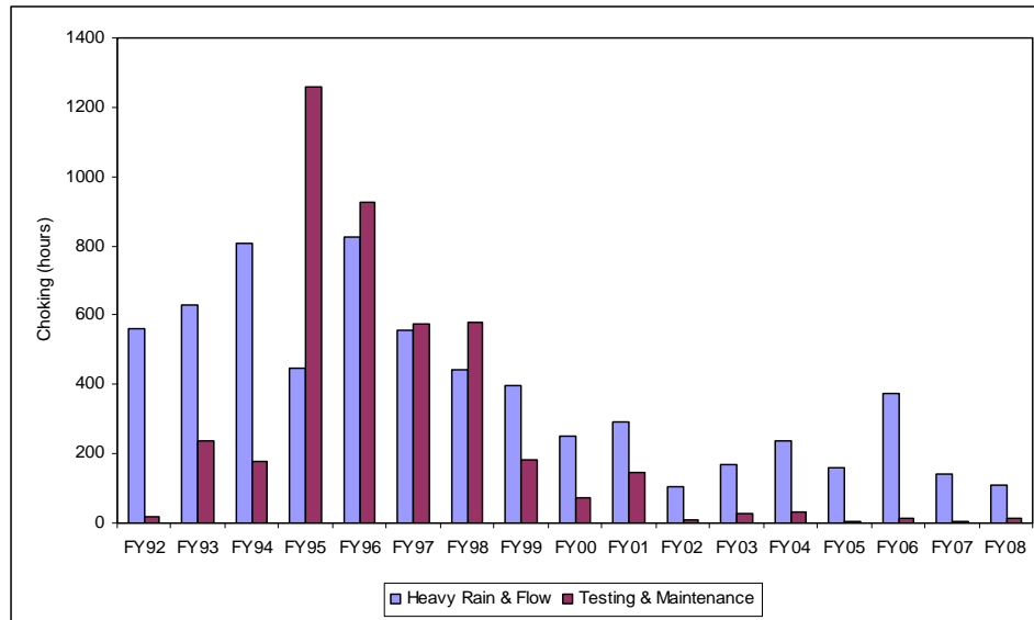
Figure 8. Headworks Choking, FY92-FY08
