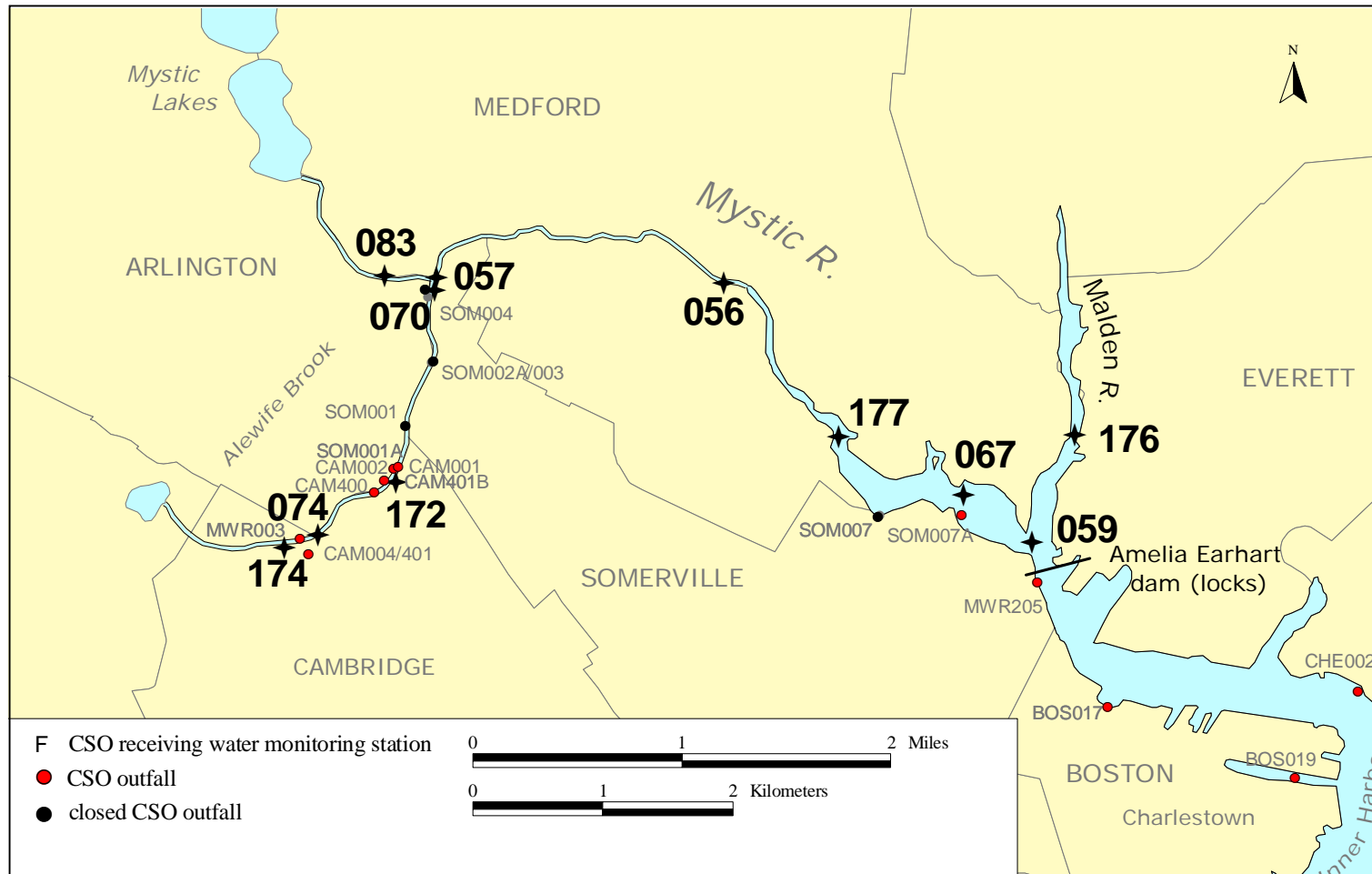
Figure 1. Sampling locations for Alewife Brook/Upper Mystic River CSO receiving water monitoring
