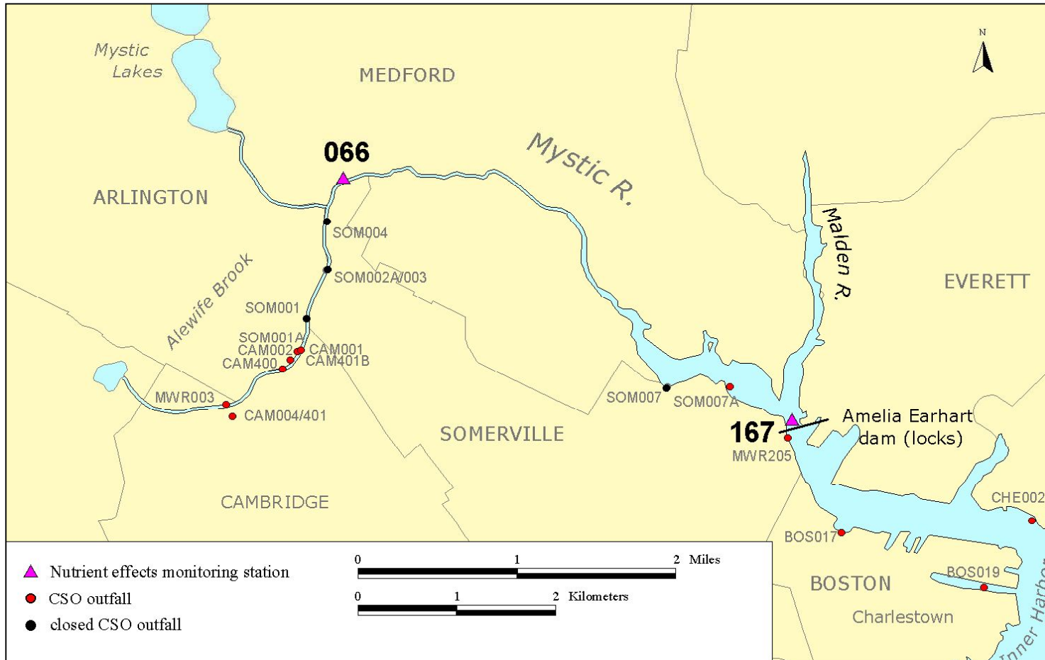
Figure 2. Sampling locations for Alewife Brook/Upper Mystic River nutrient effects monitoring
