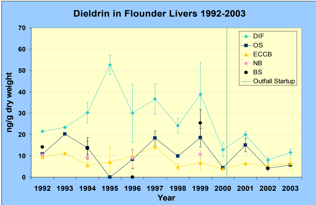
Figure D - 13. Dieldrin in Flounder Livers at the Five Collection Sites from 1992-2003.
