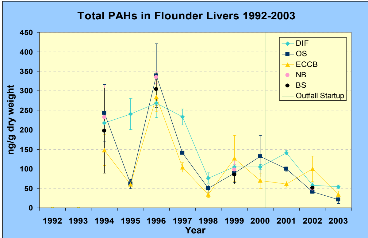
Figure D - 11. Total PAH in Flounder Livers at the Five Collection Sites from 1992-2003.
