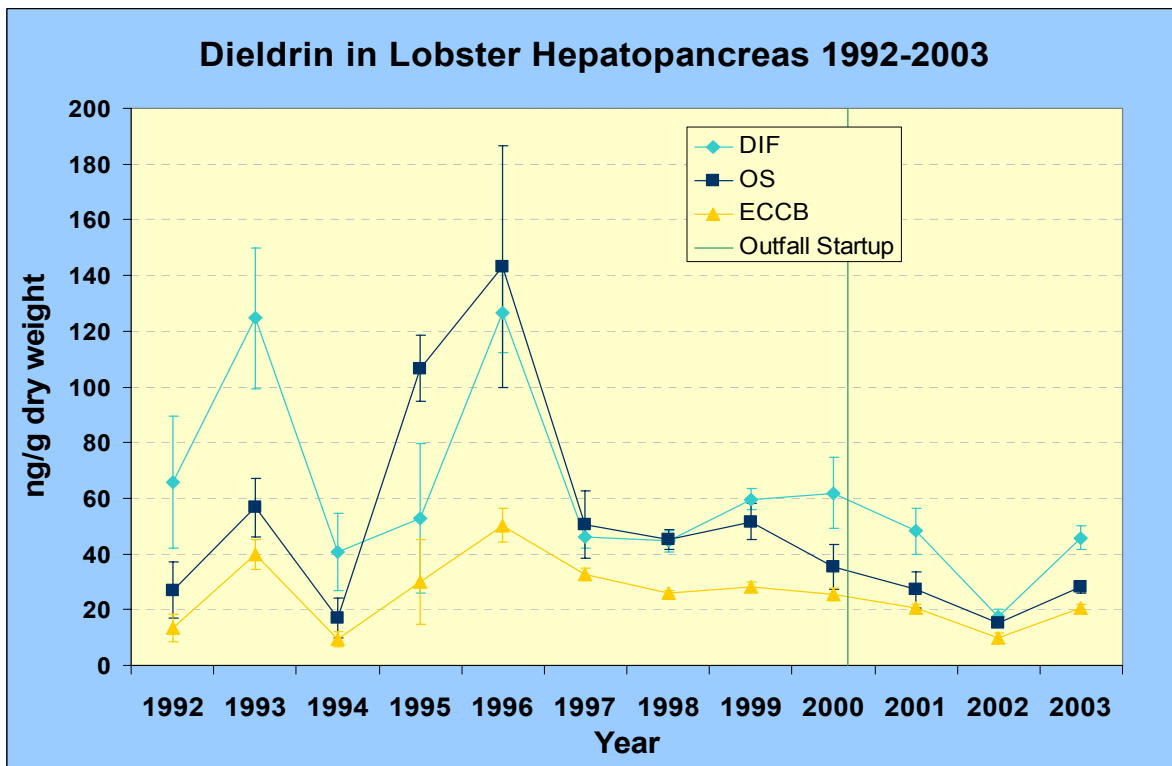
Figure D - 26. Dieldrin in Lobster Hepatopancreas at DIF, OS, and ECCB from 1992-2003.
