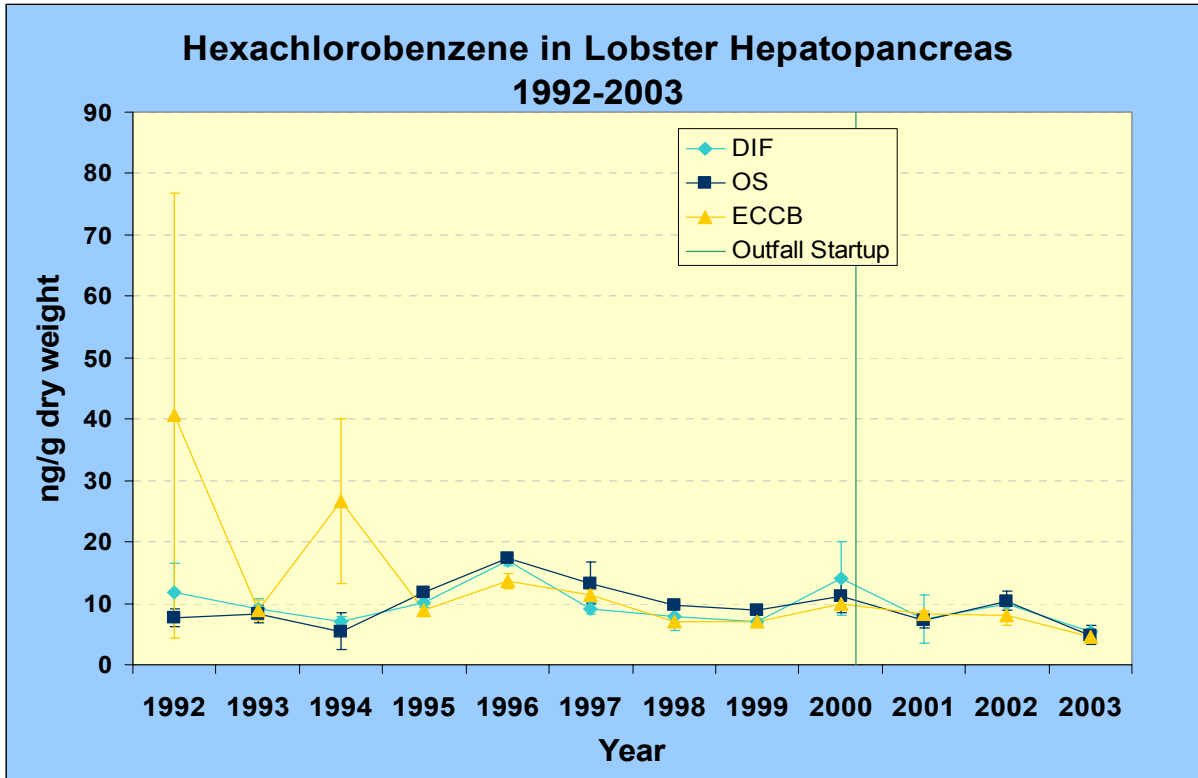
Figure D - 27. Hexachlorobenzene in Lobster Hepatopancreas at DIF, OS, and ECCB from 1992-2003.
