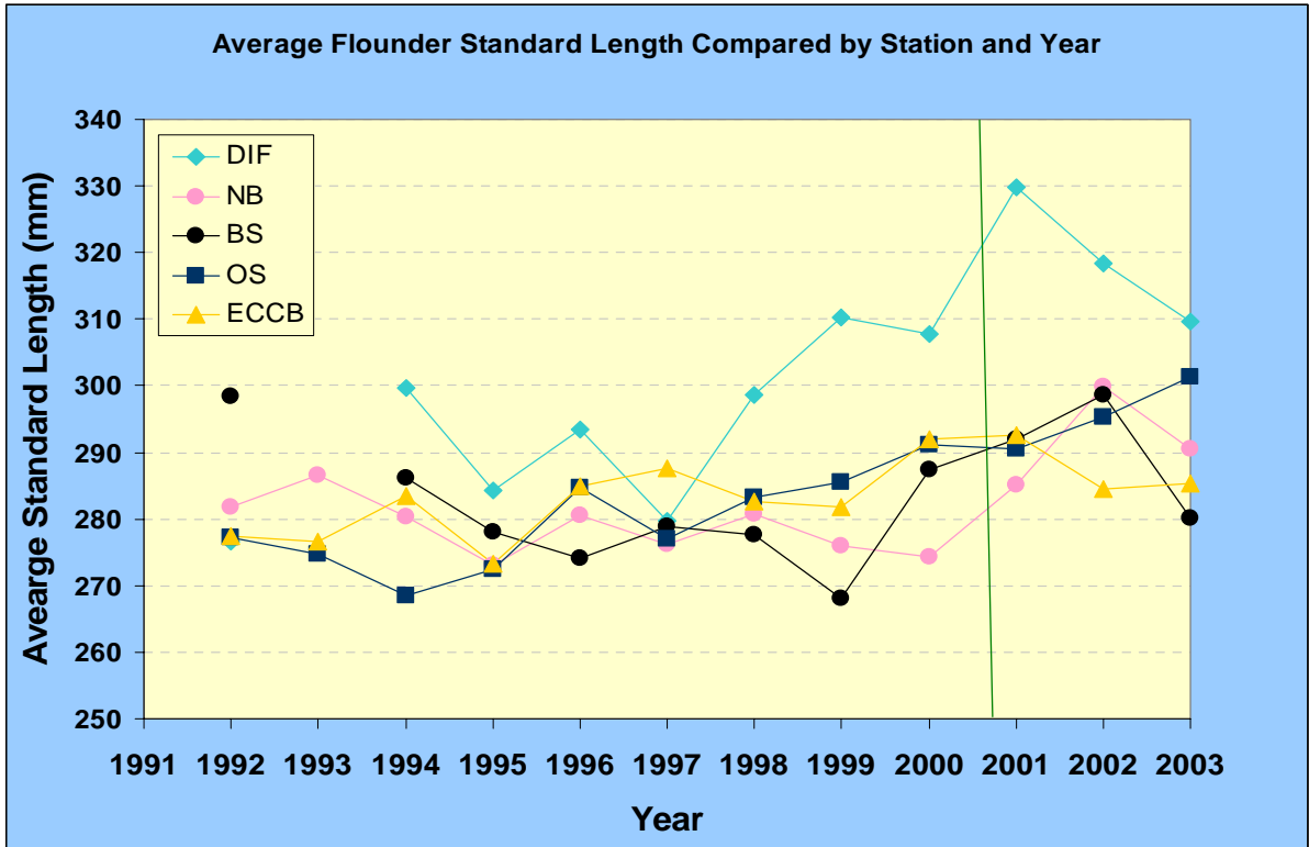
Figure 3-7. Average Flounder Standard Length Compared by Station and Year.
