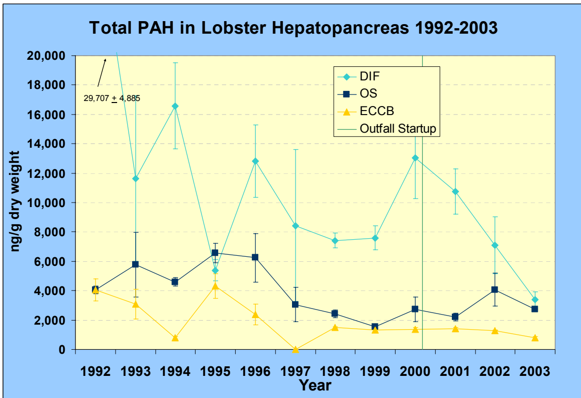
Figure D - 24. Total PAH in Lobster Hepatopancreas at DIF, OS, and ECCB from 1992-2003.
