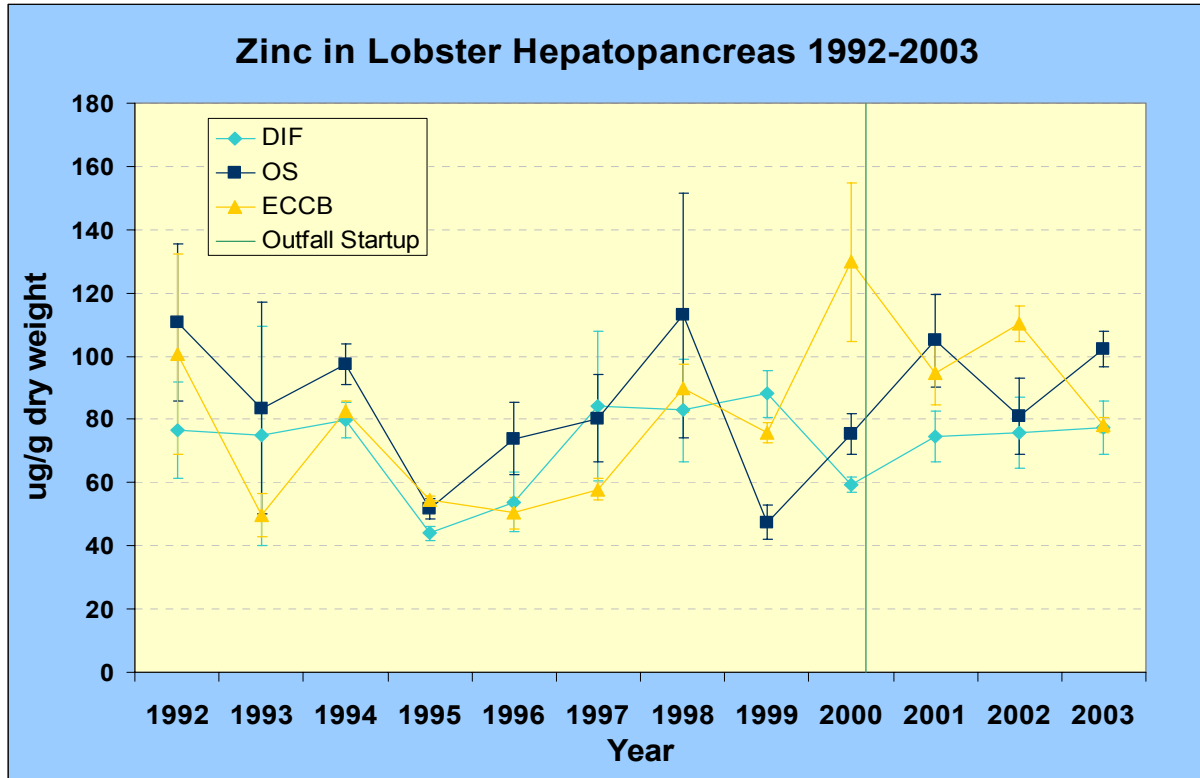
Figure D - 23. Zinc in Lobster Hepatopancreas at DIF, OS, and ECCB from 1992-2003.
