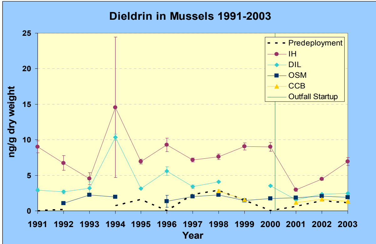
Figure D - 31. Dieldrin in Pre-deployed and Deployed Mussels from 1991-2003.
