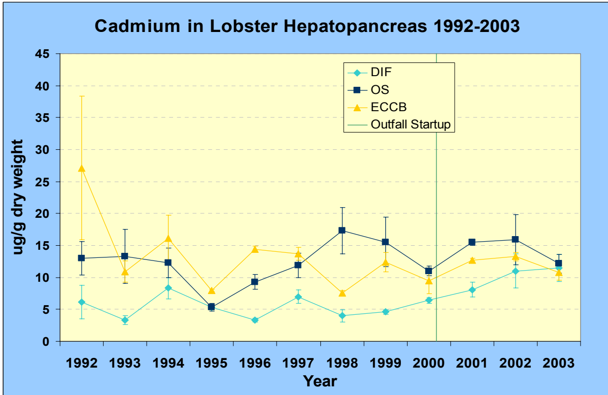
Figure D - 19. Cadmium in Lobster Hepatopancreas at DIF, OS, and ECCB from 1992-2003.
