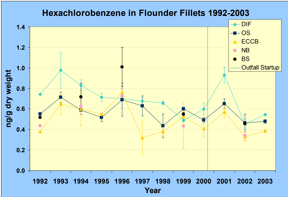
Figure D - 3. Hexachlorobenzene in Flounder Fillets at the Five Collection Sites from 1992-2003.
