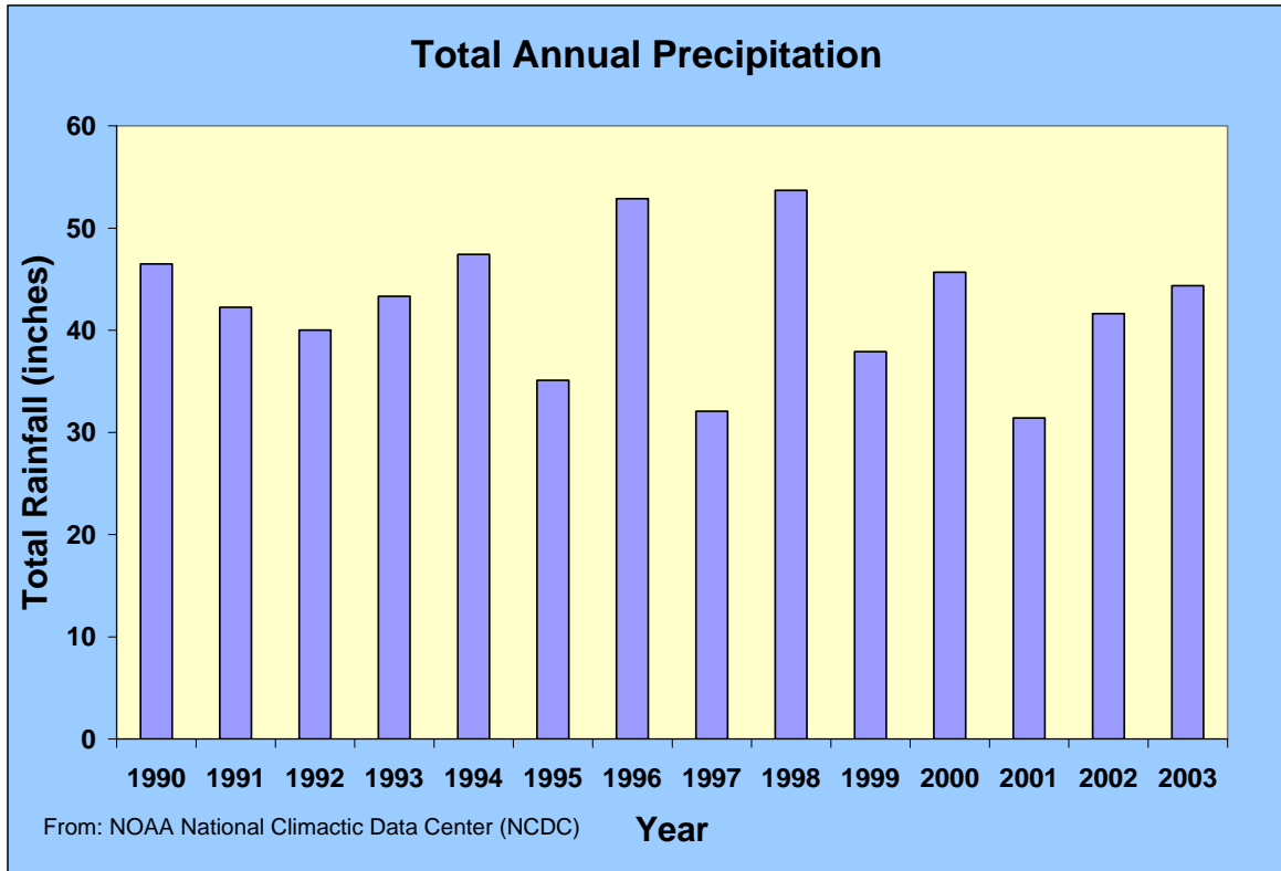
Figure 3-37. Total Annual Precipitation for Boston, MA.
